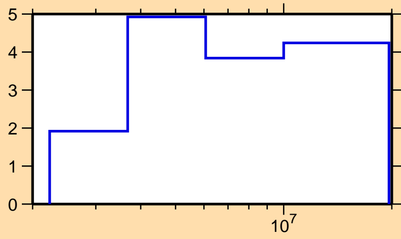
\Delta\sigma/\sigma vs. E for ^{91}\text{Y}(n,tot.)
