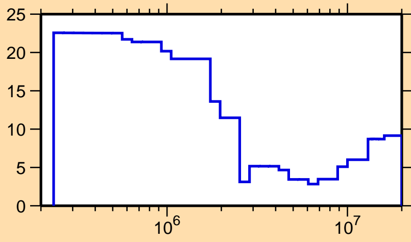
\Delta\sigma/\sigma vs. E for ^{92}\text{Y}(n,\text{tot.})
