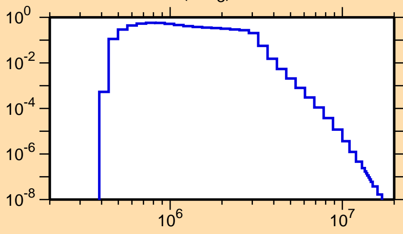
\sigma vs. E for ^{92}\text{Y}(n,n_3)
