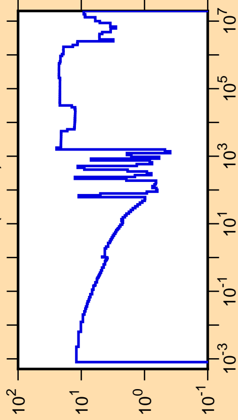
\Delta\sigma/\sigma vs. E for ^{92}\text{Y}(n,\text{tot.})
