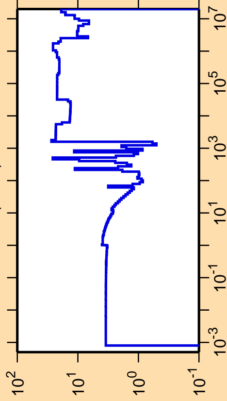
\Delta\sigma/\sigma vs. E for ^{92}\text{Y}(n,\text{el.})
