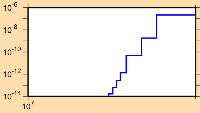
\sigma vs. E for ^{92}\text{Y}(n,2n\alpha)
