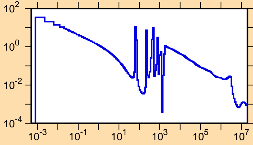
\sigma vs. E for ^{92}\text{Y}(n,\gamma)
