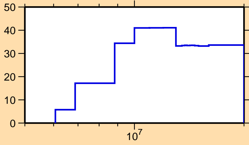
\Delta\sigma/\sigma vs. E for ^{92}\text{Y}(n,\text{inel.})
