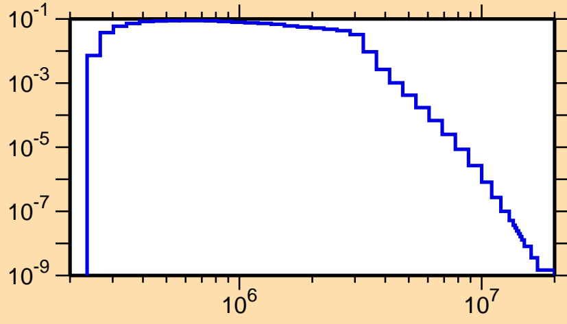
\sigma vs. E for ^{92}\text{Y}(n,n_1)
