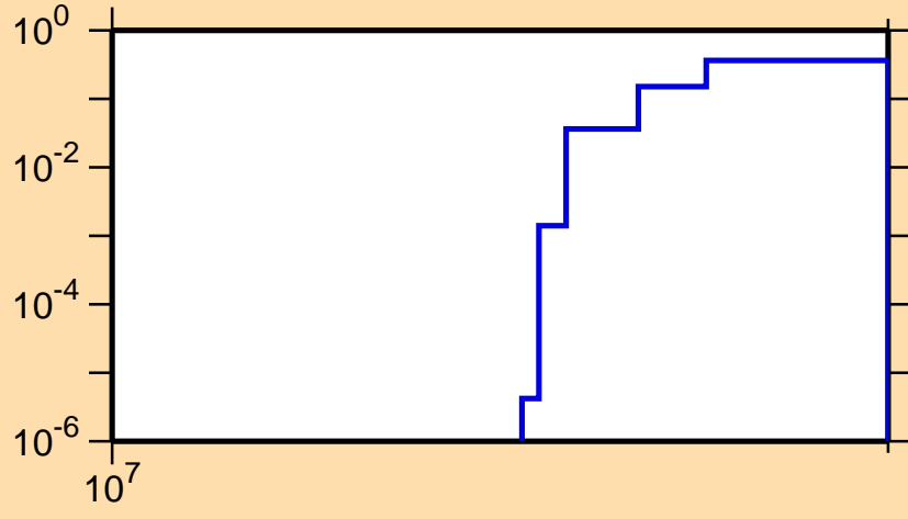
\sigma vs. E for ^{92}\text{Y}(n,3n)
