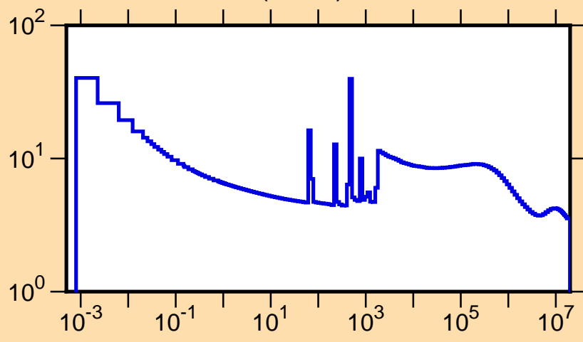
\sigma vs. E for ^{92}\text{Y}(n,\text{tot.})
