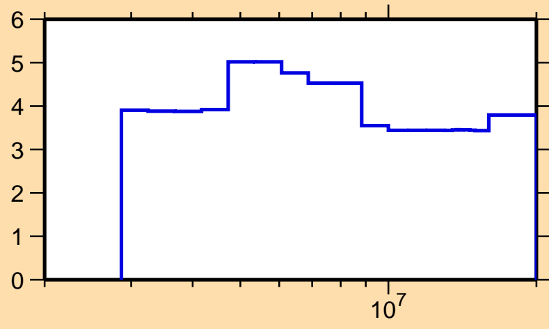
\Delta\sigma/\sigma vs. E for ^{92}\text{Y}(n,n\text{onel.})
