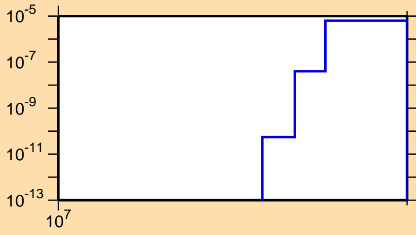
\sigma vs. E for ^{92}\text{Y}(n,nt)
