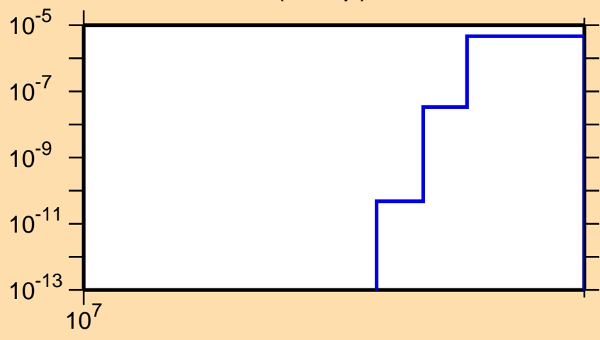
\sigma vs. E for ^{92}\text{Y}(n,2np)
