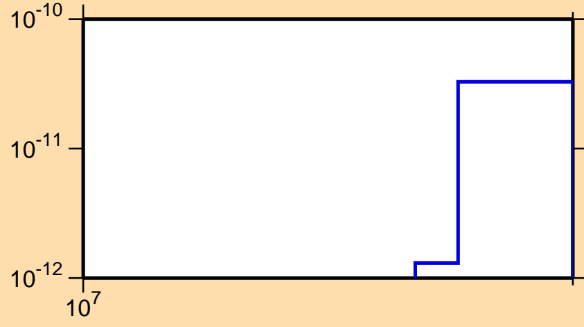
\sigma vs. E for ^{92}\text{Y}(n,p\alpha)
