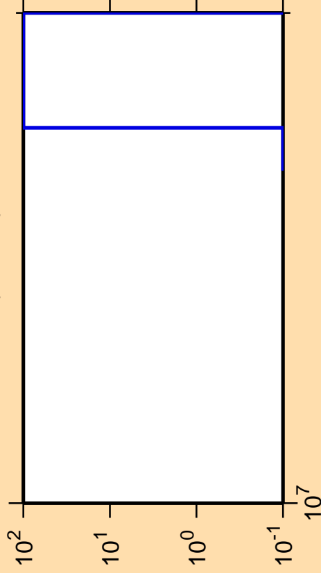
\Delta\sigma/\sigma vs. E for ^{92}\text{Y}(n,\text{He}3)
