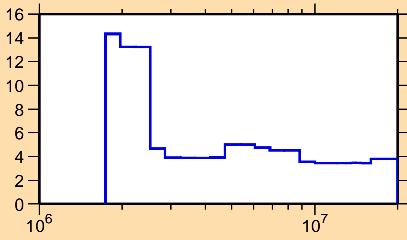
\Delta\sigma/\sigma vs. E for ^{92}\text{Y}(n,\text{nonel.})
