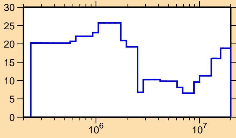
\Delta\sigma/\sigma vs. E for ^{92}\text{Y}(n,\text{el.})
