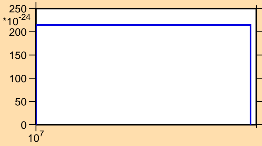
\sigma vs. E for ^{92}\text{Y} (mt 34)
