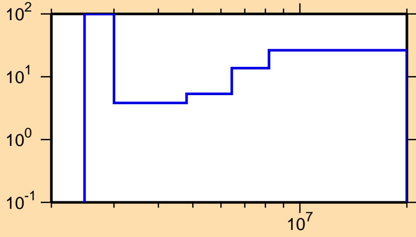
\Delta\sigma/\sigma vs. E for ^{92}\text{Y}(n,ncont.)
