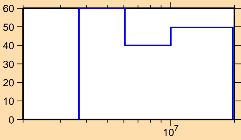
\Delta\sigma/\sigma vs. E for ^{93}\text{Y}(n,p)
