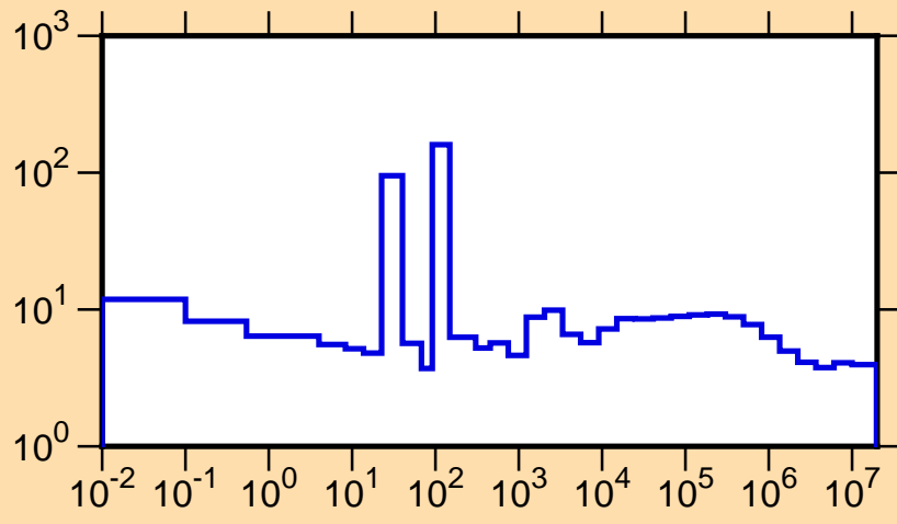
\sigma vs. E for ^{93}\text{Y}(n,\text{tot.})
