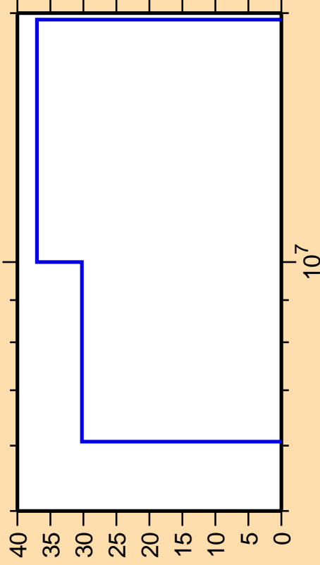
\Delta\sigma/\sigma vs. E for ^{93}\text{Y}(n,n_1)
