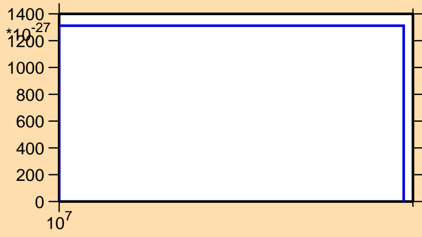
\sigma vs. E for ^{93}\text{Y}(n,3n\alpha)
