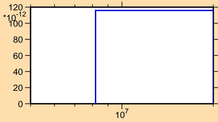
\sigma vs. E for ^{93}\text{Y}(n,2n\alpha)
