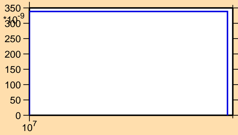
\sigma vs. E for ^{94}\text{Y}(n,nd)
