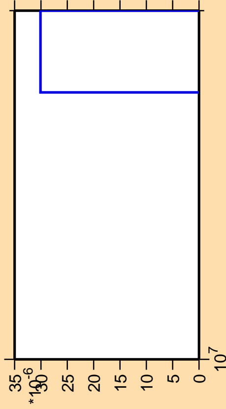
\Delta\sigma/\sigma vs. E for ^{95}\text{Y}(n,3n\alpha)
