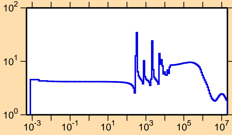
\sigma vs. E for ^{95}\text{Y}(n,\text{el.})
