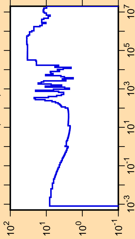
\Delta\sigma/\sigma vs. E for ^{95}\text{Y}(n,\text{tot.})
