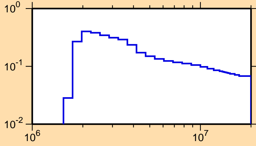
\sigma vs. E for ^{95}\text{Y}(n,n_4)
