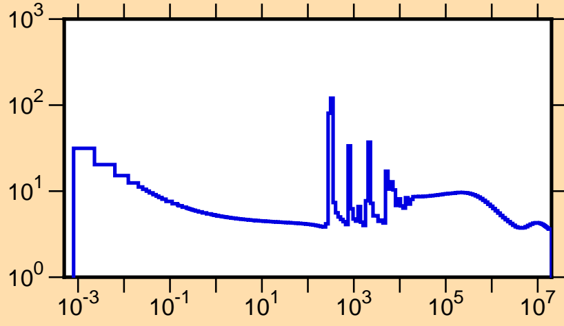
\sigma vs. E for ^{95}\text{Y}(n,\text{tot.})
