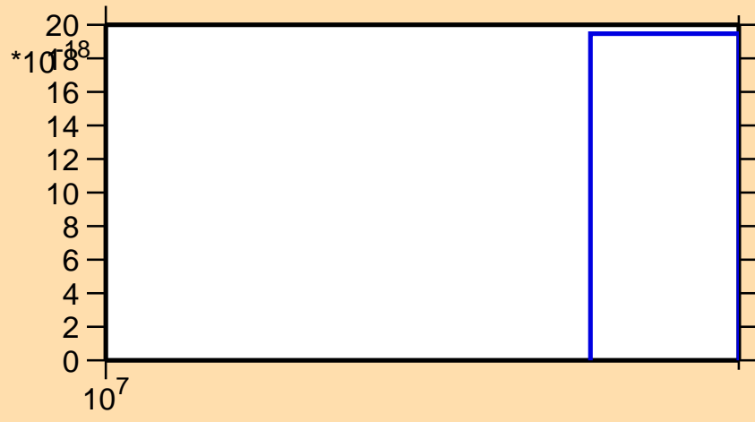
\sigma vs. E for ^{95}\text{Y}(n,3n\alpha)
