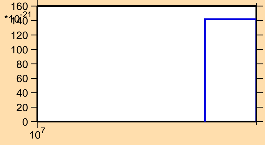
\sigma vs. E for ^{95}\text{Y} (mt 11)
