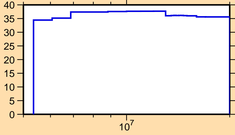
\Delta\sigma/\sigma vs. E for ^{95}\text{Y}(n,n_1)
