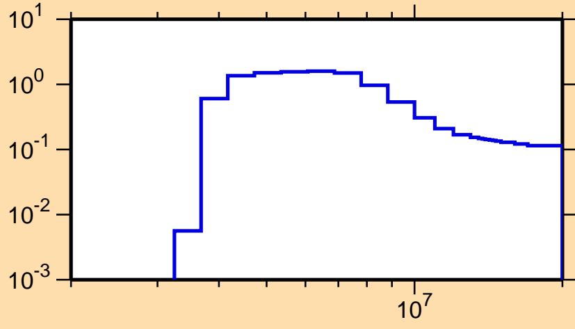
\sigma vs. E for ^{95}\text{Y}(n,n\text{cont.})
