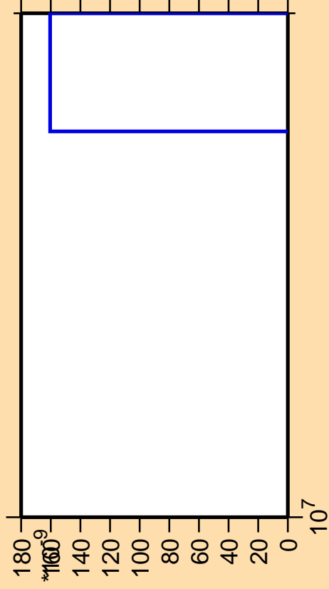
\Delta\sigma/\sigma vs. E for ^{95}\text{Y} (mt 11)
