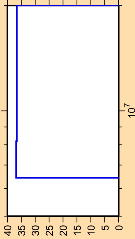
\Delta\sigma/\sigma vs. E for ^{95}\text{Y}(n,n_1)
