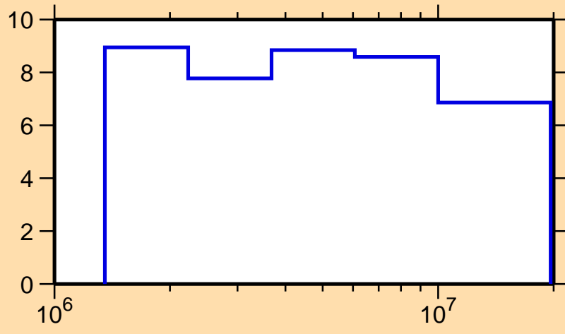
\Delta\sigma/\sigma vs. E for ^{96}\text{Y}(n,n\text{onel.})
