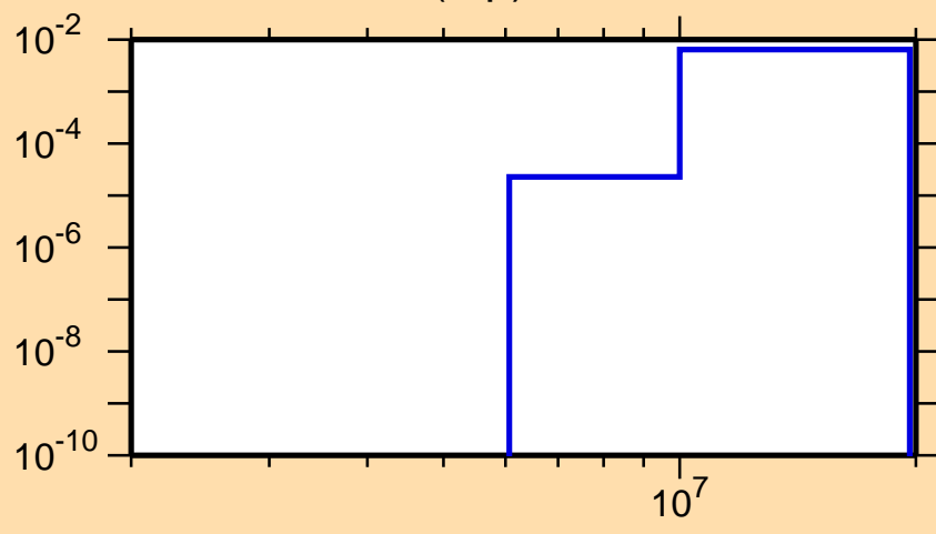
\sigma vs. E for ^{96}\text{Y}(n,p)
