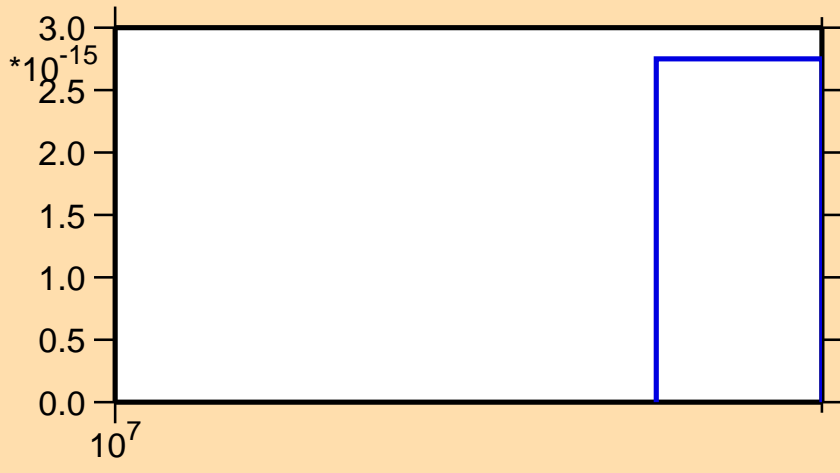
\sigma vs. E for ^{96}\text{Y} (mt 11)
