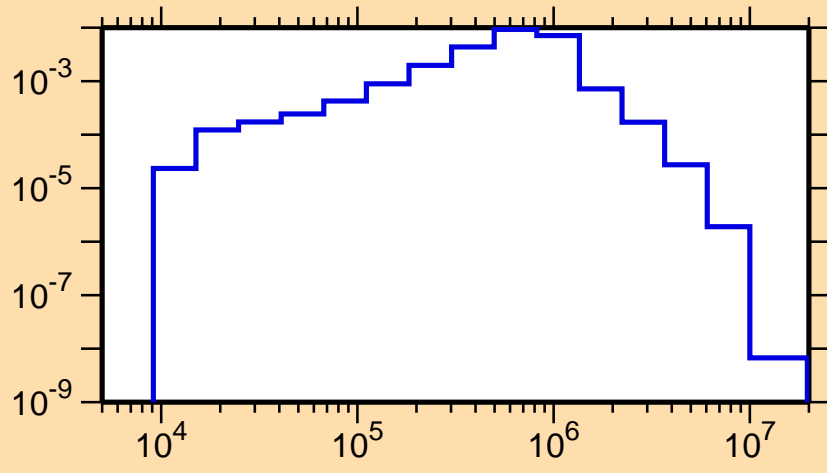
\sigma vs. E for ^{96}\text{Y}(n,n_4)
