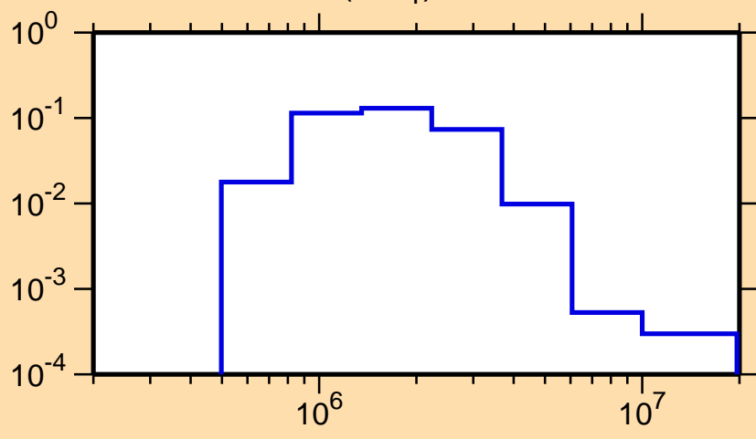
\sigma vs. E for ^{97}\text{Y}(n,n_1)
