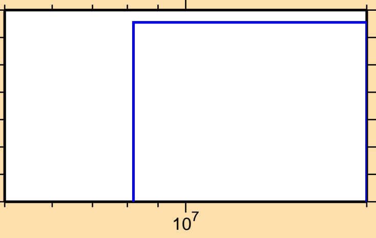
\sigma vs. E for ^{97}\text{Y}(n,\text{nd})
