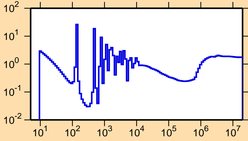
\sigma vs. E for ^{97}\text{Y}(n,\text{nonel.})
