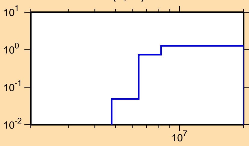
\sigma vs. E for ^{97}\text{Y}(n,2n)
