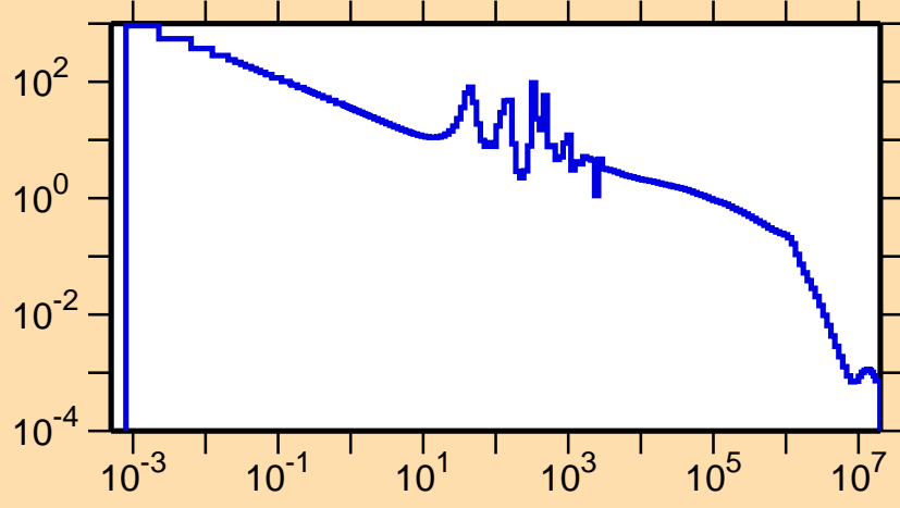
\sigma vs. E for ^{98}\text{Y}(n,\gamma)
