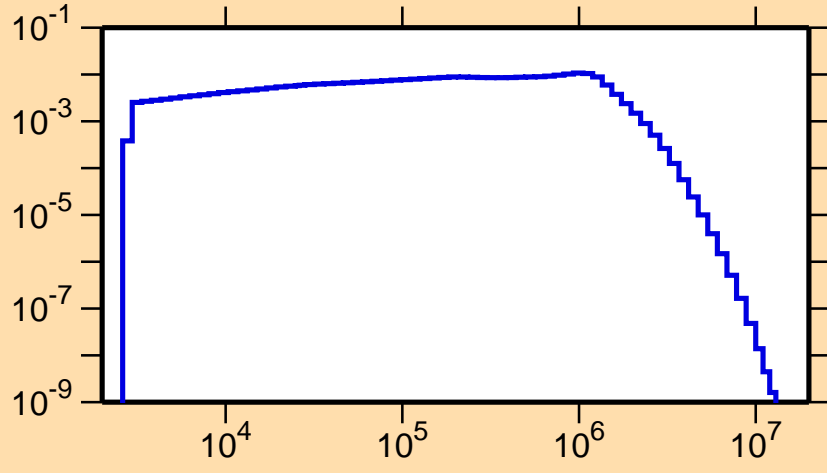
\sigma vs. E for ^{98}\text{Y}(n,n_1)
