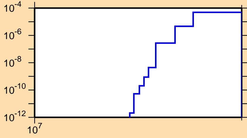
\sigma vs. E for ^{98}\text{Y}(n,nd)
