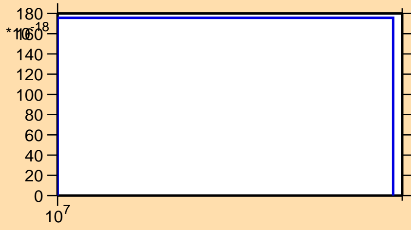
\sigma vs. E for ^{98}\text{Y} (mt 11)
