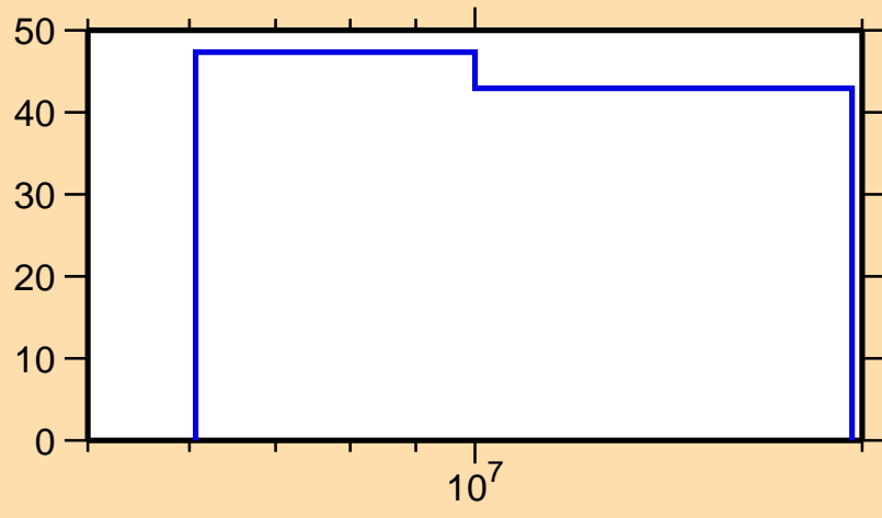
\Delta\sigma/\sigma vs. E for ^{98}\text{Y}(n,p)
