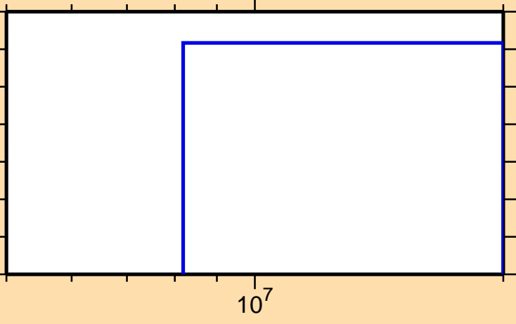
\sigma vs. E for ^{98}\text{Y}(n,n\alpha)
