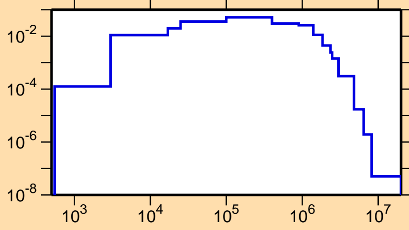
\sigma vs. E for ^{98}\text{Y}(n,n_4)
