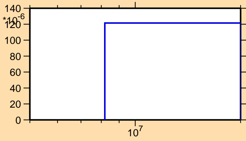
\sigma vs. E for ^{98}\text{Y}(n,d)
