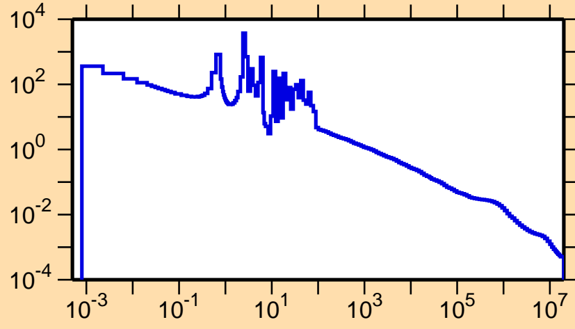
\sigma vs. E for ^{151}\text{Yb}(n,\gamma)
