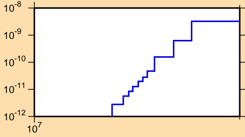
\sigma vs. E for ^{151}\text{Yb}(\text{mt117})
