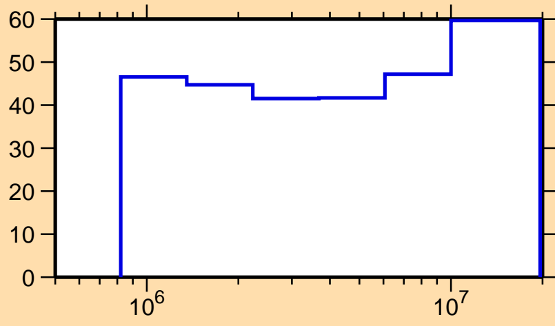
\Delta\sigma/\sigma vs. E for ^{151}\text{Yb}(n,n_1)
