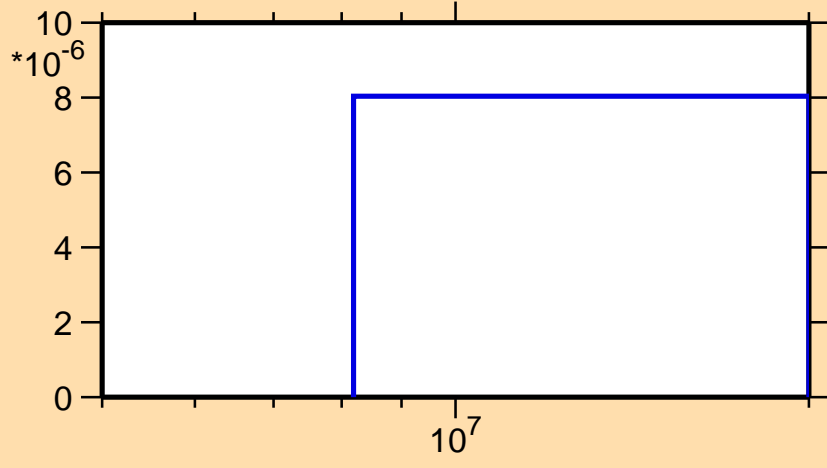
\sigma vs. E for ^{151}\text{Yb}(n,\text{pt})
