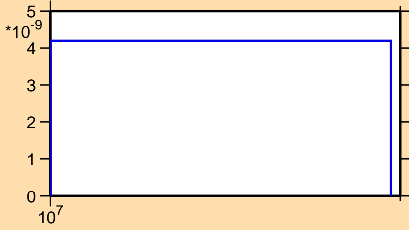
\sigma vs. E for ^{153}\text{Yb}(n,2n\alpha)
