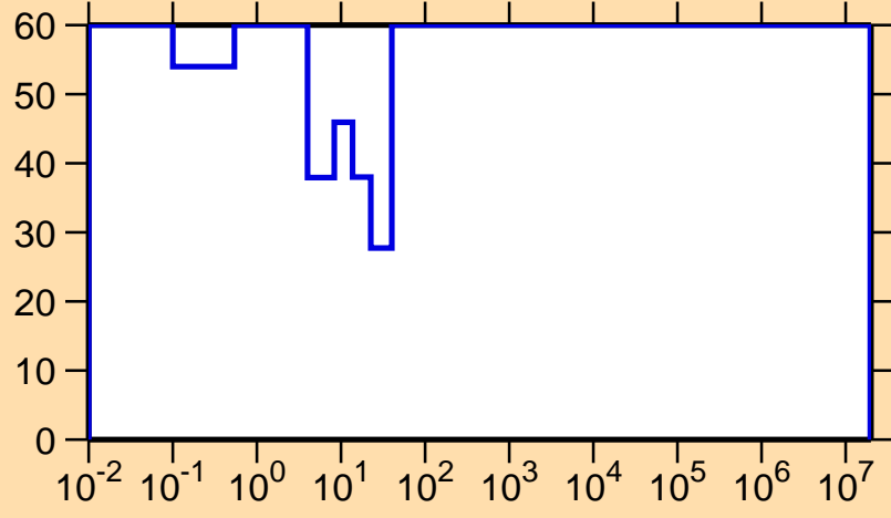
\Delta\sigma/\sigma vs. E for ^{153}\text{Yb}(n,\gamma)
