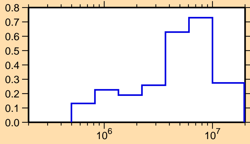
\sigma vs. E for ^{153}\text{Yb}(n,\text{inel.})
