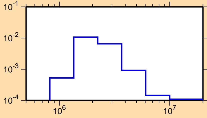
\sigma vs. E for ^{153}\text{Yb}(n,n_2)
