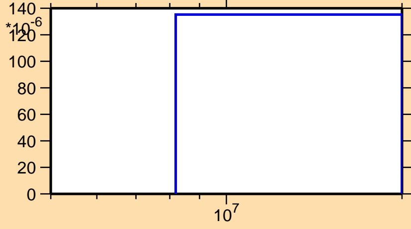
\sigma vs. E for ^{153}\text{Yb}(n,2np)
