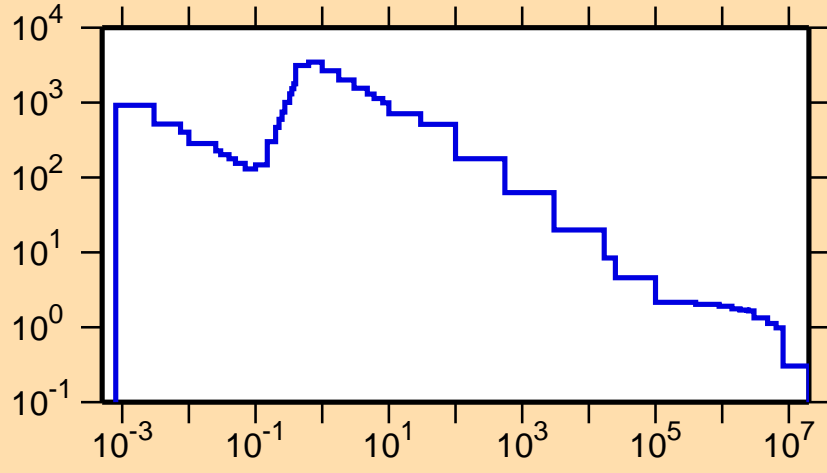
\sigma vs. E for ^{153}\text{Yb}(n,p)
