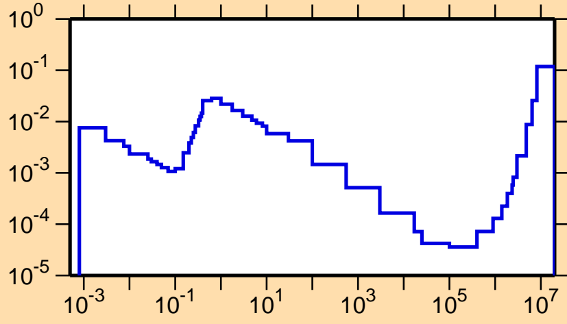
\sigma vs. E for ^{153}\text{Yb}(n,p\alpha)
