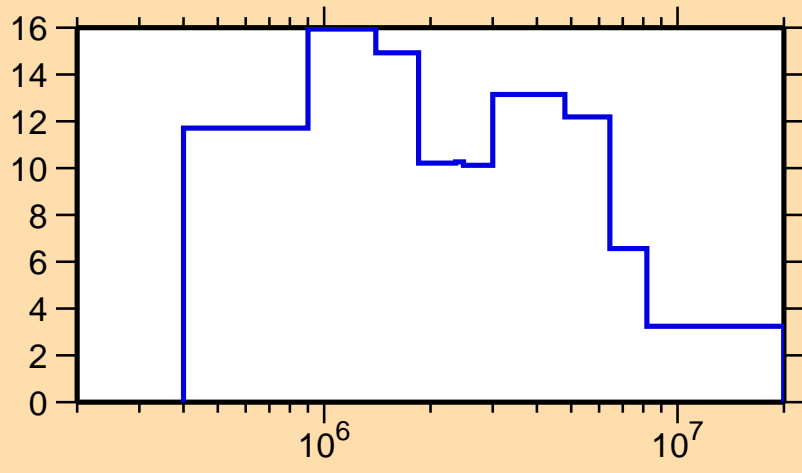
\Delta\sigma/\sigma vs. E for ^{153}\text{Yb}(n,\text{tot.})
