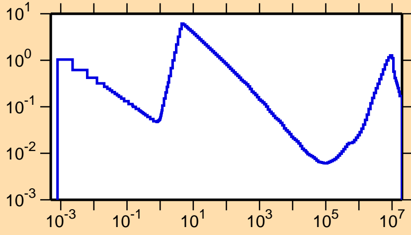
\sigma vs. E for ^{156}\text{Yb}(n,p)
