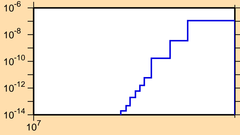
\sigma vs. E for ^{156}\text{Yb}(n,\text{pt})
