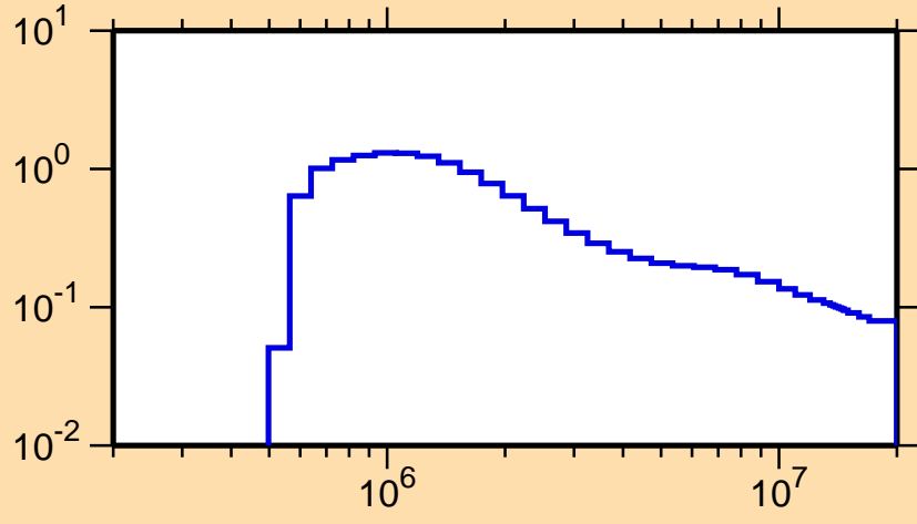
\sigma vs. E for ^{156}\text{Yb}(n,n_1)
