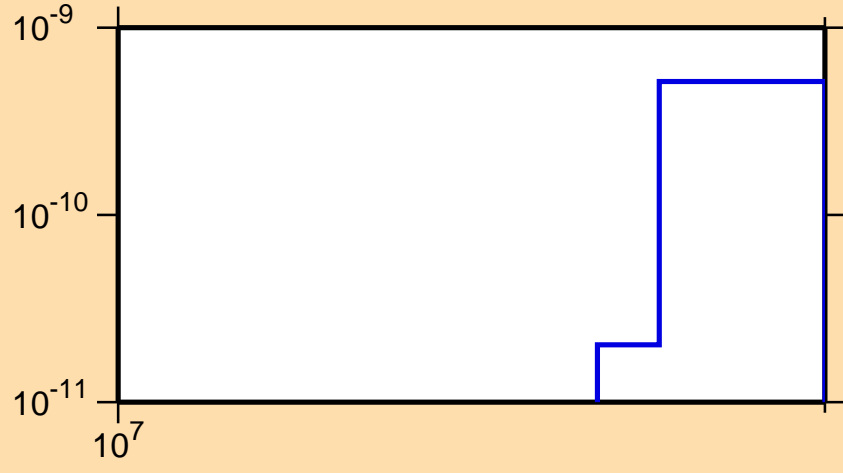
\sigma vs. E for ^{156}\text{Yb} (mt 34)
