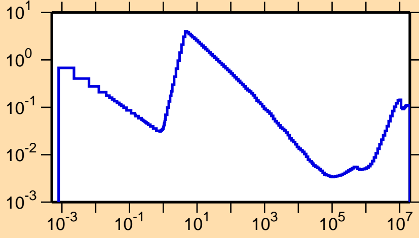
\sigma vs. E for ^{156}\text{Yb}(n,\alpha)
