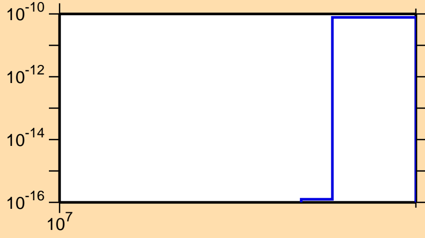
\sigma vs. E for ^{156}\text{Yb}(n,nt)
