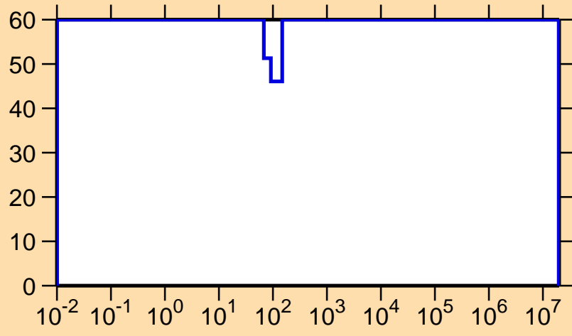
\Delta\sigma/\sigma vs. E for ^{156}\text{Yb}(n,\gamma)
