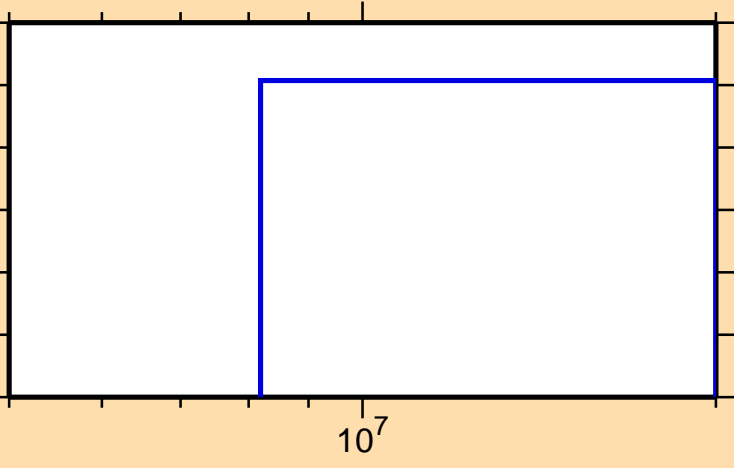
\sigma vs. E for ^{156}\text{Yb}(n,t)
