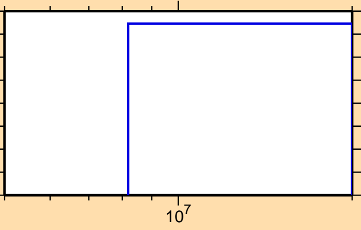
\sigma vs. E for ^{156}\text{Yb}(n,2n\alpha)
