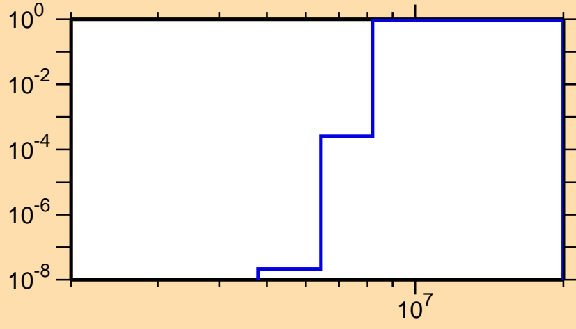
\sigma vs. E for ^{156}\text{Yb}(n,np)
