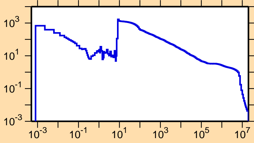
\sigma vs. E for ^{157}\text{Yb}(n,\gamma)
