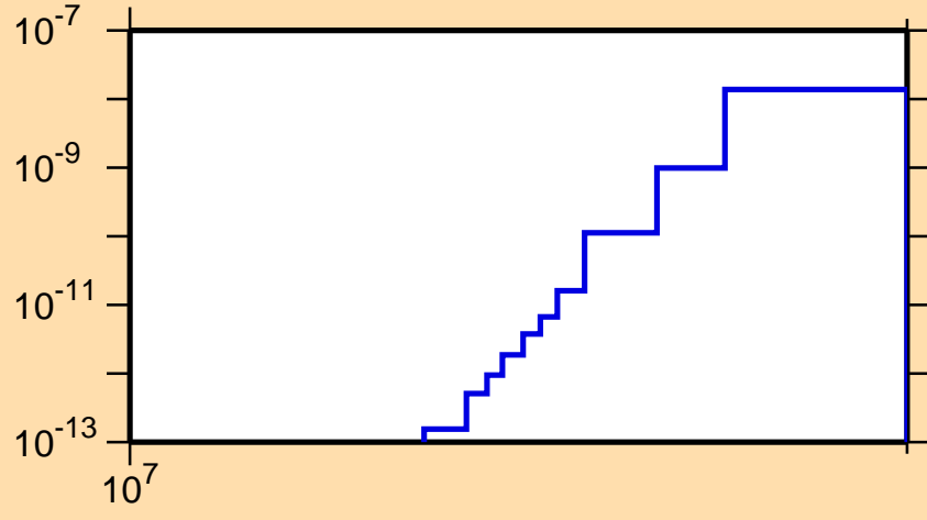
\sigma vs. E for ^{157}\text{Yb} (mt 34)
