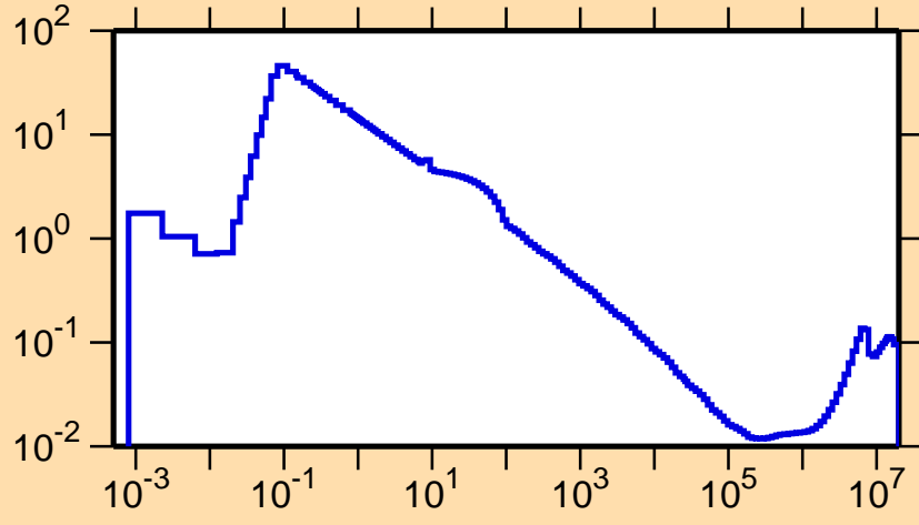
\sigma vs. E for ^{157}\text{Yb}(n,\alpha)
