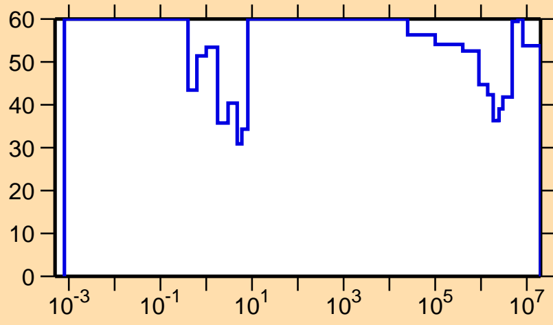
\Delta\sigma/\sigma vs. E for ^{157}\text{Yb}(n,\gamma)
