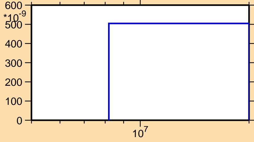
\sigma vs. E for ^{157}\text{Yb}(n,\text{pd})
