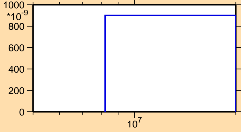
\sigma vs. E for ^{157}\text{Yb} (mt 45)
