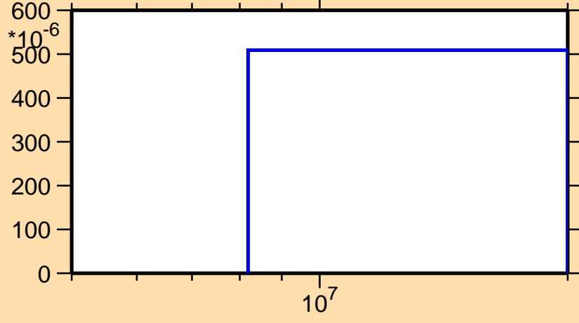
\sigma vs. E for ^{157}\text{Yb}(n,2n\alpha)
