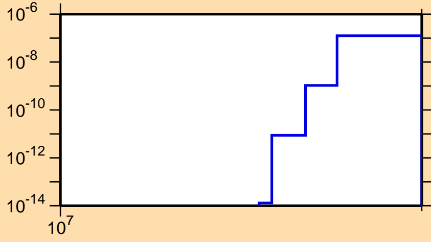
\sigma vs. E for ^{158}\text{Yb}(n,nd)
