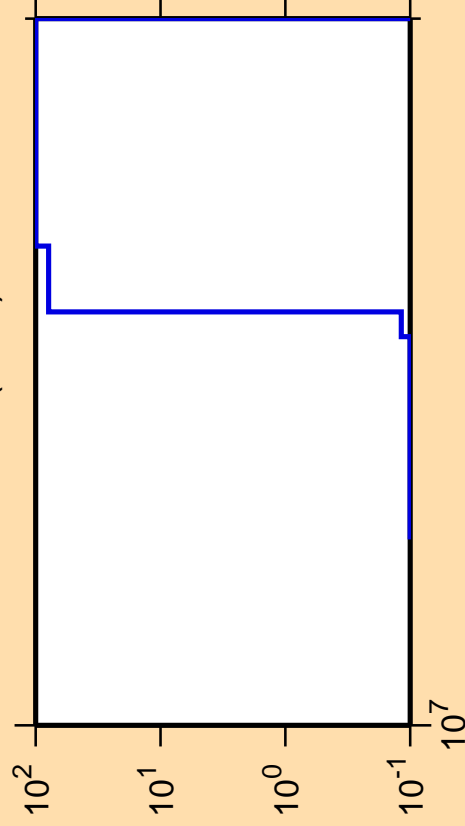
\Delta\sigma/\sigma vs. E for ^{158}\text{Yb}(n,nd)
