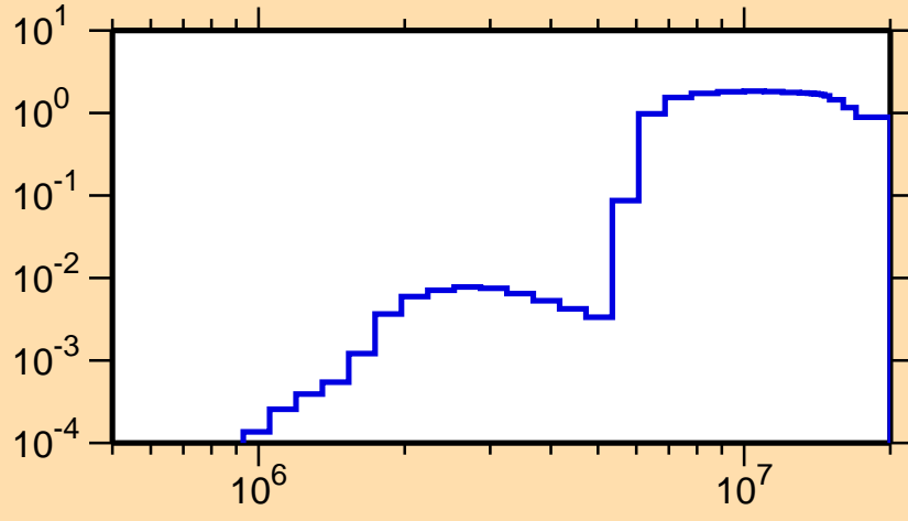
\sigma vs. E for ^{158}\text{Yb}(n,n\text{cont.})
