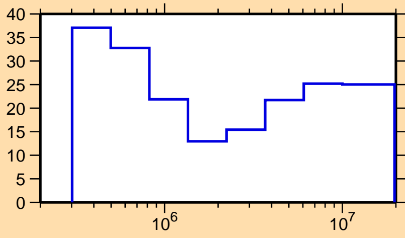
\Delta\sigma/\sigma vs. E for ^{158}\text{Yb}(n,\text{nonel.})
