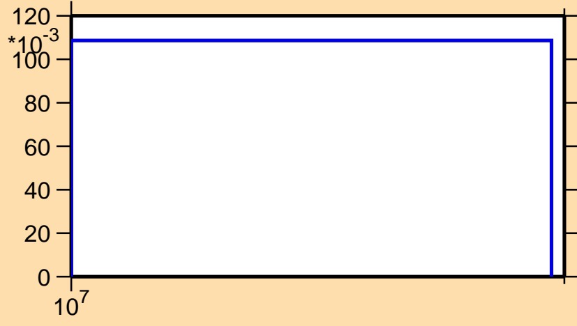
\sigma vs. E for ^{158}\text{Yb}(n,2n)
