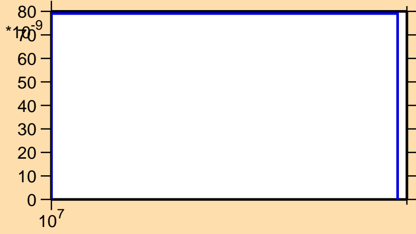
\sigma vs. E for ^{158}\text{Yb}(n,3n)
