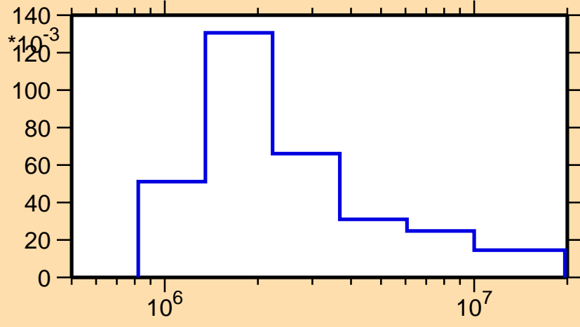
\sigma vs. E for ^{158}\text{Yb}(n,n_2)
