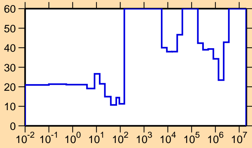
\Delta\sigma/\sigma vs. E for ^{158}\text{Yb}(n,\gamma)
