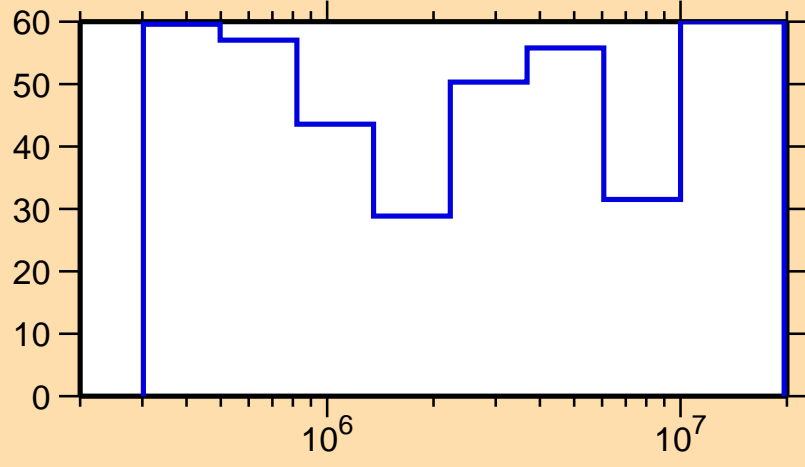
\Delta\sigma/\sigma vs. E for ^{158}\text{Yb}(n,n_1)
