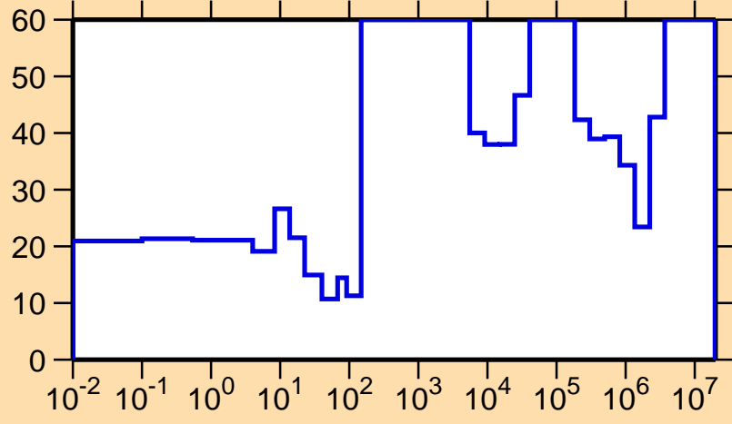
\Delta\sigma/\sigma vs. E for ^{158}\text{Yb}(n,\gamma)
