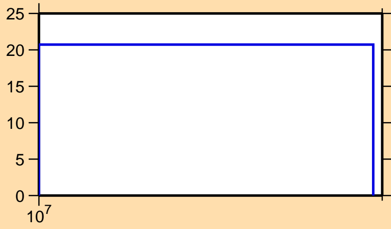
\Delta\sigma/\sigma vs. E for ^{158}\text{Yb}(n,\text{tot.})
