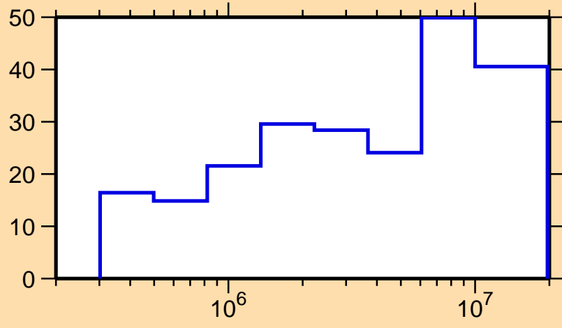
\Delta\sigma/\sigma vs. E for ^{158}\text{Yb}(n,\text{el.})
