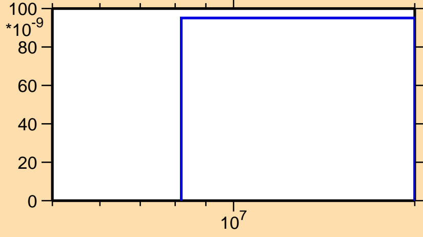
\sigma vs. E for ^{158}\text{Yb}(n,\text{pd})
