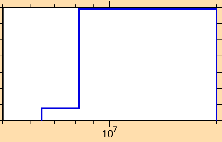
\sigma vs. E for ^{158}\text{Yb}(n,\text{He}3)
