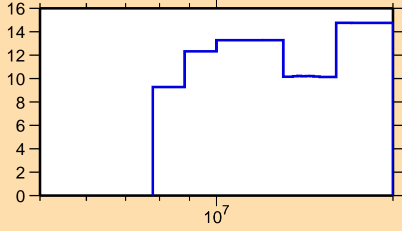
\Delta\sigma/\sigma vs. E for ^{159}\text{Yb}(n,\text{nonel.})
