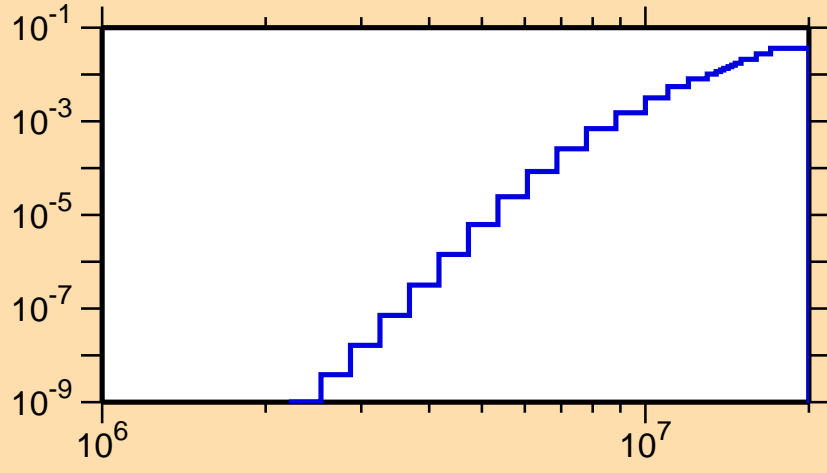
\sigma vs. E for ^{159}\text{Yb}(n,n\alpha)
