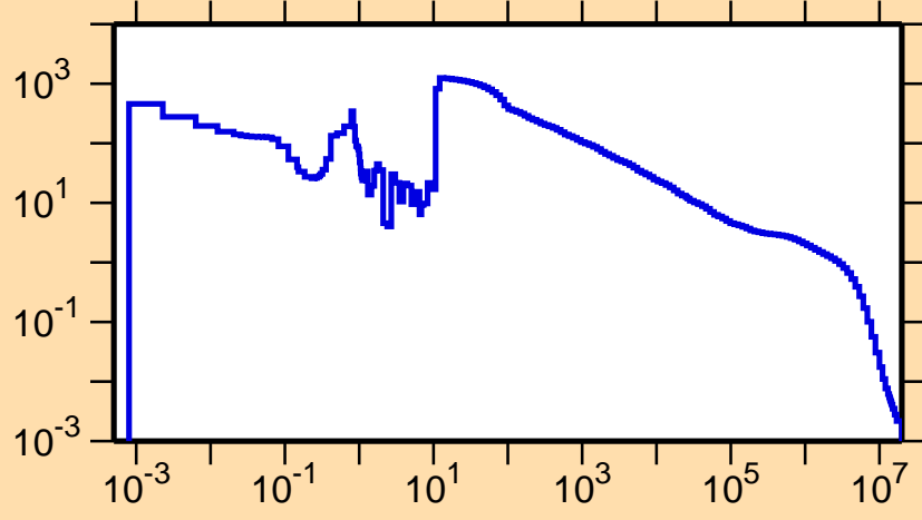
\sigma vs. E for ^{159}\text{Yb}(n,\gamma)
