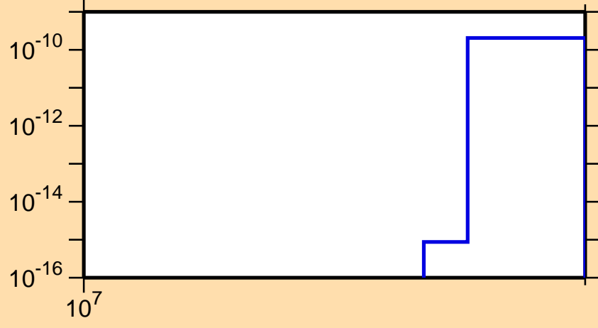
\sigma vs. E for ^{159}\text{Yb}(n,nt)
