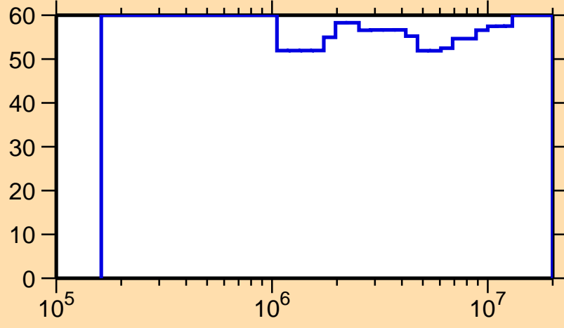
\Delta\sigma/\sigma vs. E for ^{159}\text{Yb}(n,n_1)
