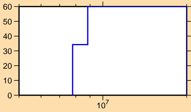
\Delta\sigma/\sigma vs. E for ^{159}\text{Yb}(n,\text{inel.})
