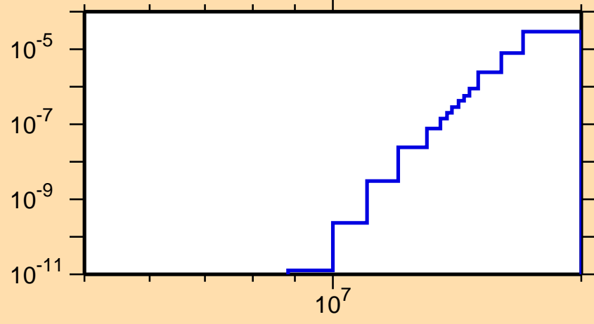
\sigma vs. E for ^{159}\text{Yb}(n,\text{He}3)
