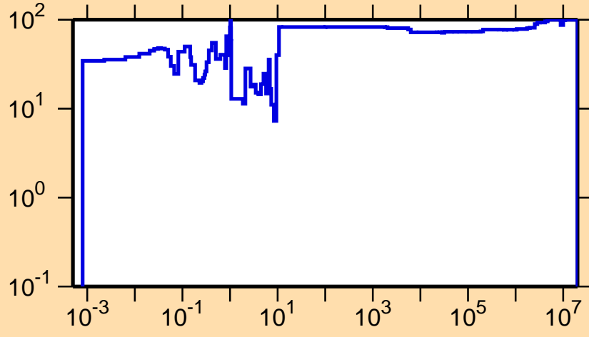
\Delta\sigma/\sigma vs. E for ^{159}\text{Yb}(n,\gamma)
