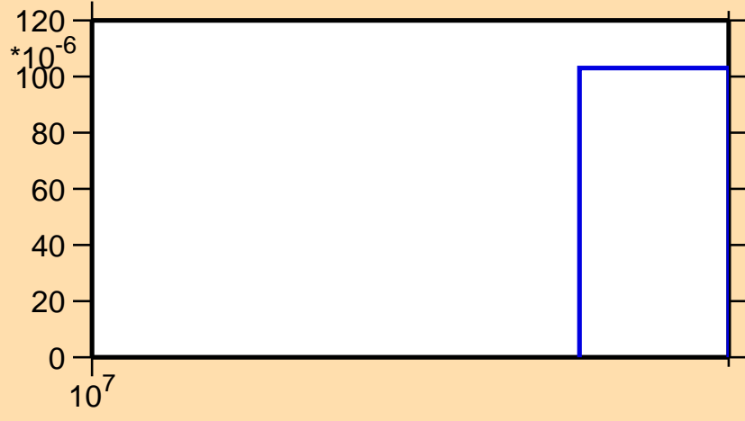
\sigma vs. E for ^{159}\text{Yb}(n,3n)
