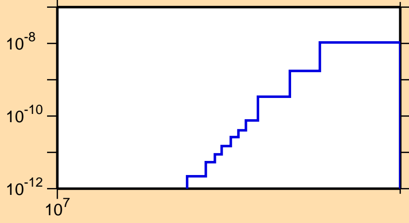
\sigma vs. E for ^{159}\text{Yb}(\text{mt117})
