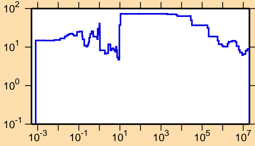
\Delta\sigma/\sigma vs. E for ^{159}\text{Yb}(n,\text{tot.})
