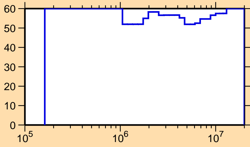
\Delta\sigma/\sigma vs. E for ^{159}\text{Yb}(n,n_1)
