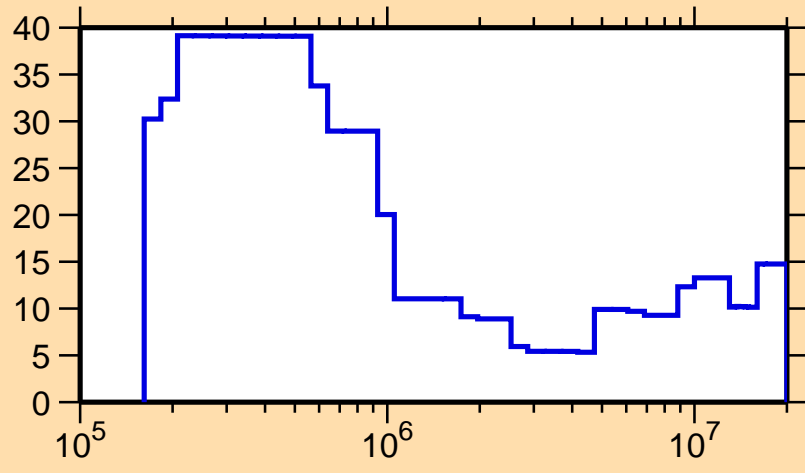
\Delta\sigma/\sigma vs. E for ^{159}\text{Yb}(n,\text{nonel.})
