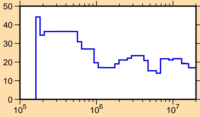
\Delta\sigma/\sigma vs. E for ^{159}\text{Yb}(n,\text{el.})
