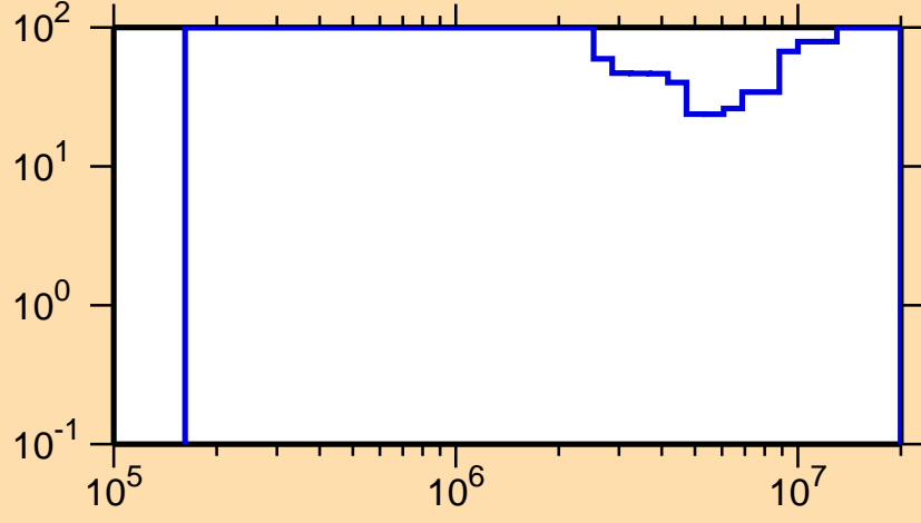
\Delta\sigma/\sigma vs. E for ^{159}\text{Yb}(n,\text{inel.})
