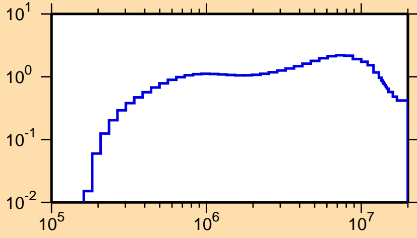
\sigma vs. E for ^{159}\text{Yb}(n,\text{inel.})
