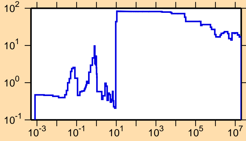
\Delta\sigma/\sigma vs. E for ^{159}\text{Yb}(n,\text{el.})
