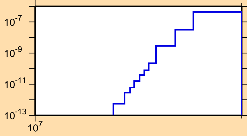
\sigma vs. E for ^{159}\text{Yb}(n,\text{pt})
