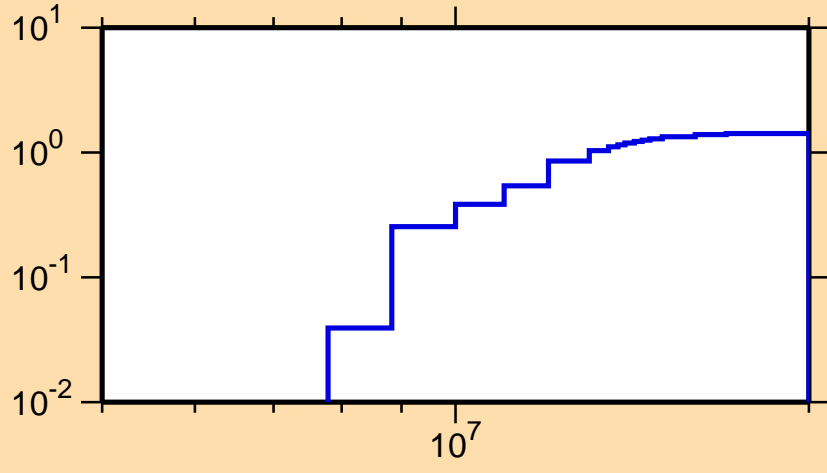
\sigma vs. E for ^{159}\text{Yb}(n,2n)
