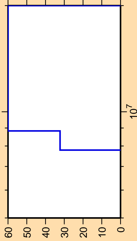
\Delta\sigma/\sigma vs. E for ^{159}\text{Yb}(n, n_{\text{cont}})
