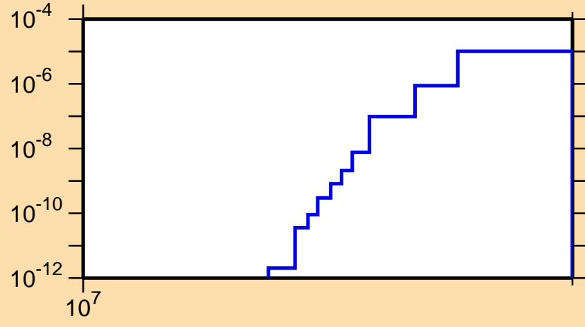
\sigma vs. E for ^{159}\text{Yb}(n,\text{nd})
