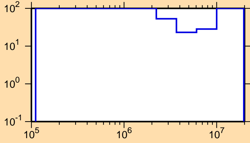
\Delta\sigma/\sigma vs. E for ^{159}\text{Yb}(n,n\text{cont.})
