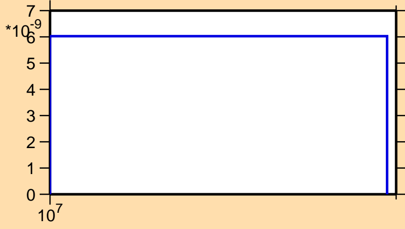
\sigma vs. E for ^{159}\text{Yb}(n,\text{pt})
