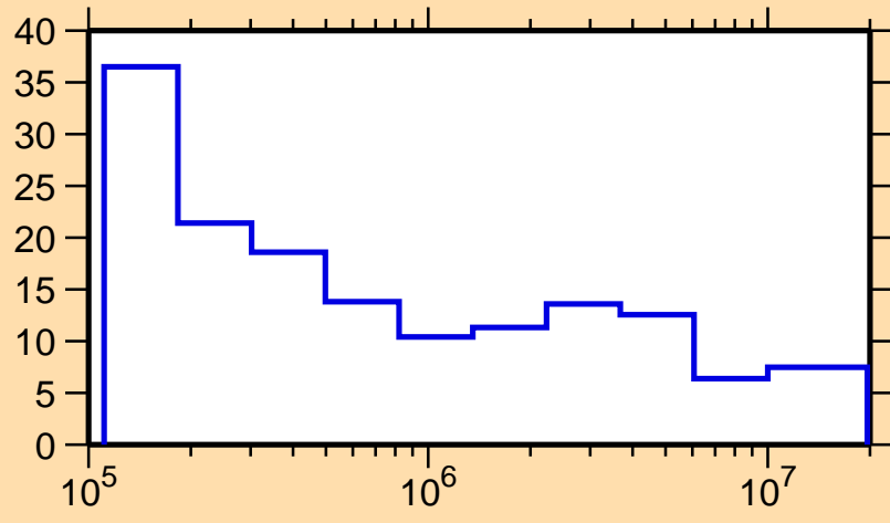
\Delta\sigma/\sigma vs. E for ^{159}\text{Yb}(n,\text{tot.})
