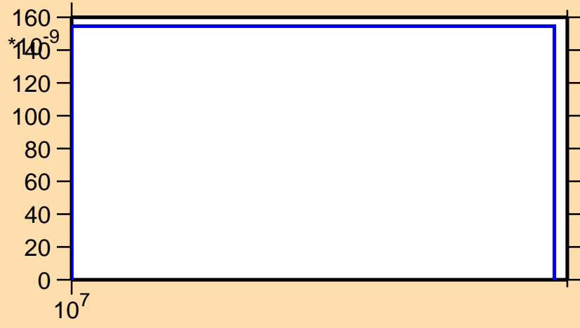
\sigma vs. E for ^{159}\text{Yb}(n,\text{nd})
