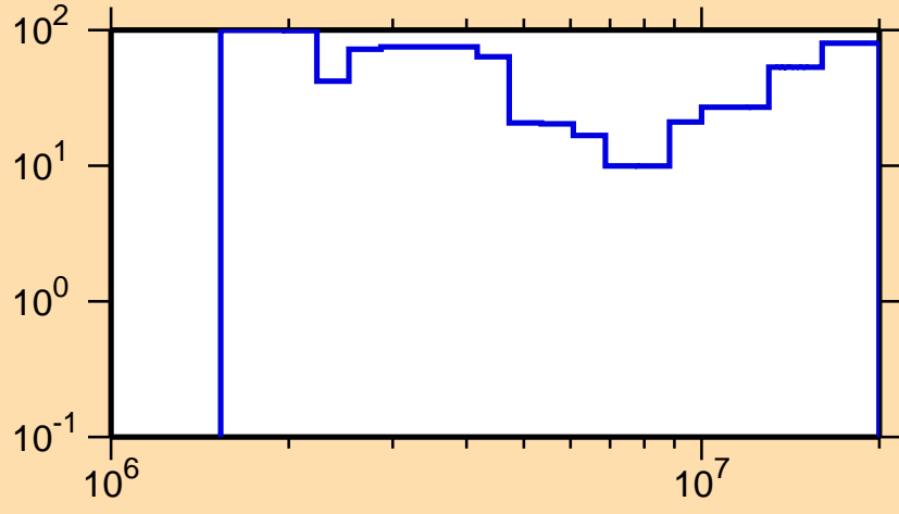
\Delta\sigma/\sigma vs. E for ^{160}\text{Yb}(n,n\text{cont.})
