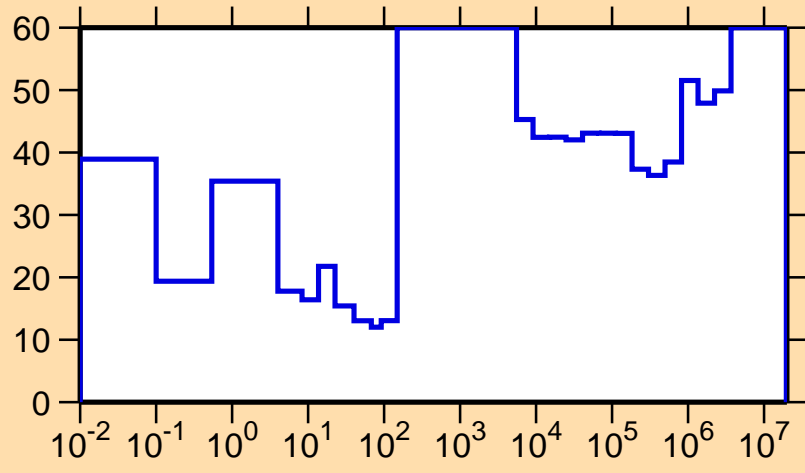
\Delta\sigma/\sigma vs. E for ^{160}\text{Yb}(n,\gamma)
