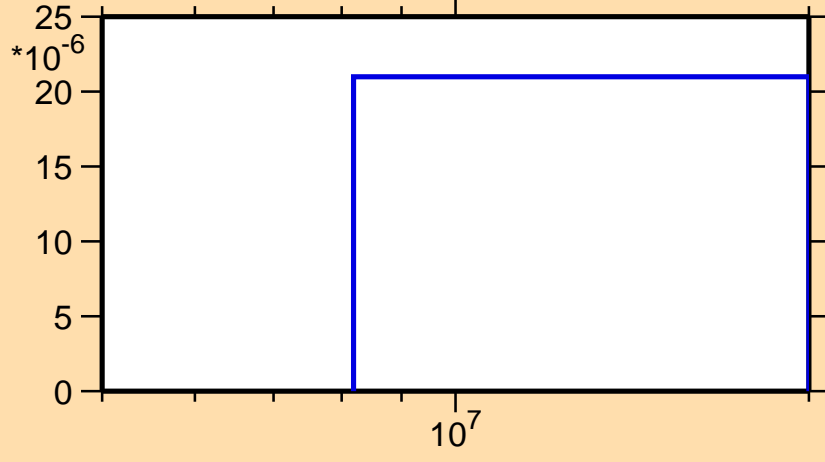
\sigma vs. E for ^{160}\text{Yb}(n,t)
