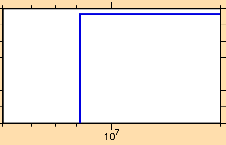
\sigma vs. E for ^{160}\text{Yb}(n,2np)
