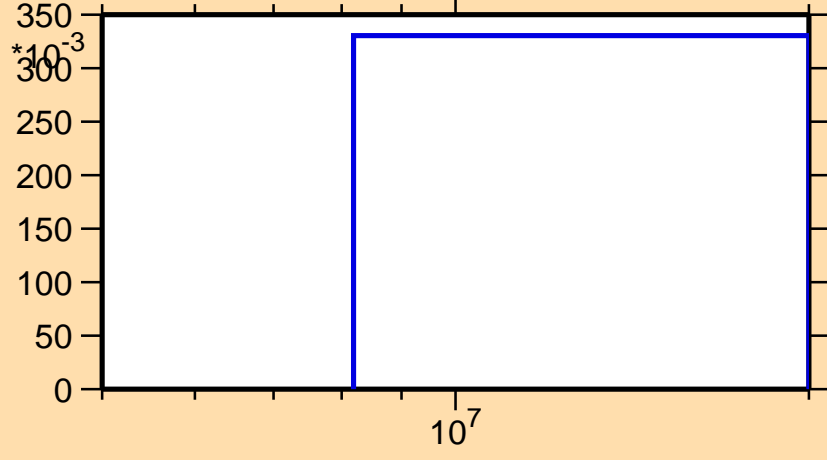
\sigma vs. E for ^{160}\text{Yb}(n,2n)
