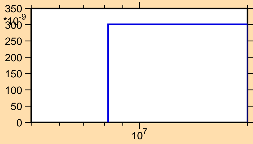
\sigma vs. E for ^{160}\text{Yb}(n,2n\alpha)
