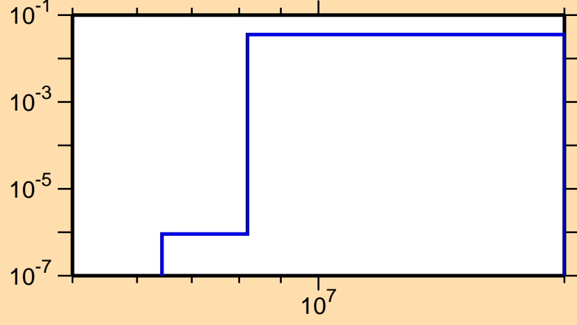
\sigma vs. E for ^{160}\text{Yb}(n,np)
