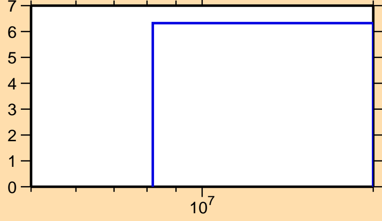
\Delta\sigma/\sigma vs. E for ^{160}\text{Yb}(n,\text{nonel.})
