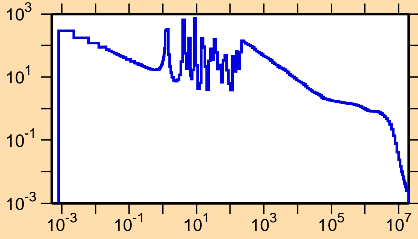
\sigma vs. E for ^{162}\text{Yb}(n,\gamma)
