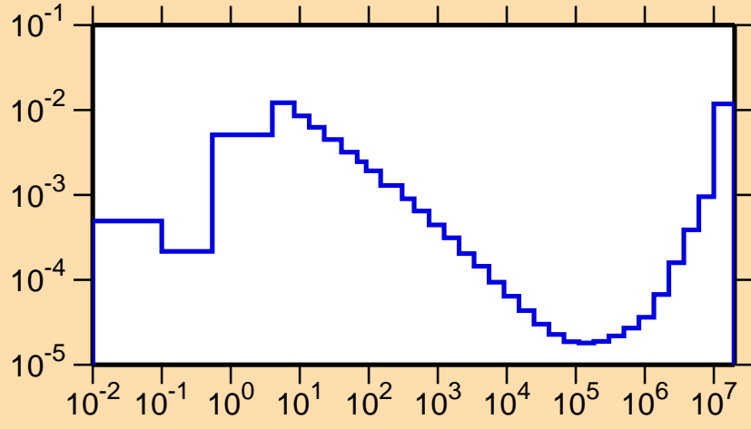
\sigma vs. E for ^{162}\text{Yb}(n,\alpha)
