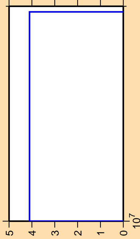
\Delta\sigma/\sigma vs. E for ^{162}\text{Yb}(n,nt)
