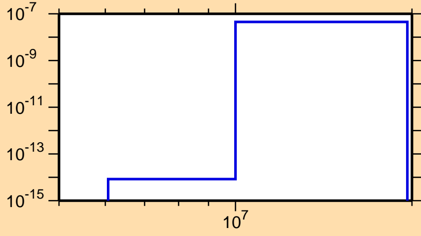
\sigma vs. E for ^{162}\text{Yb}(n,\text{He3})
