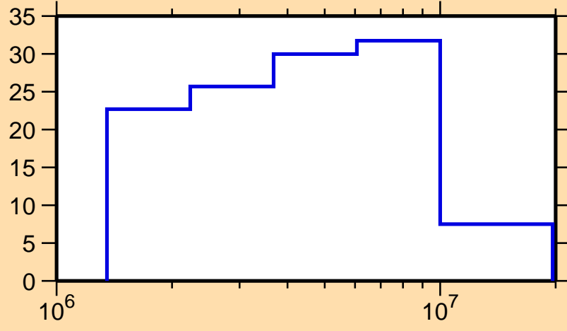
\Delta\sigma/\sigma vs. E for ^{162}\text{Yb}(n, el.)
