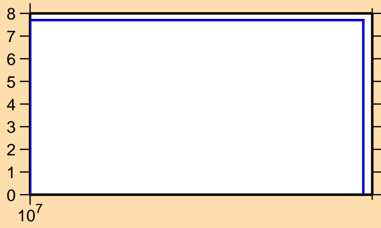
\Delta\sigma/\sigma vs. E for ^{162}\text{Yb}(n,\text{tot.})
