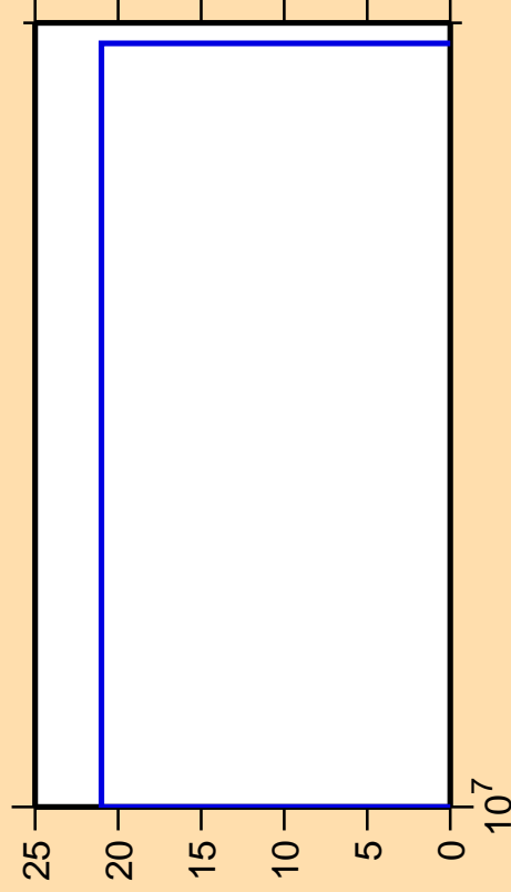
\Delta\sigma/\sigma vs. E for ^{162}\text{Yb} (mt117)
