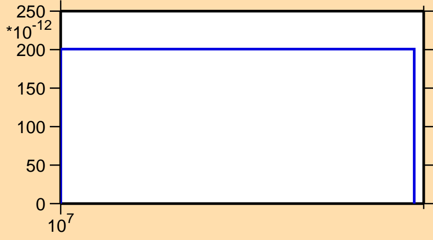
\sigma vs. E for ^{162}\text{Yb}(n,\text{pd})
