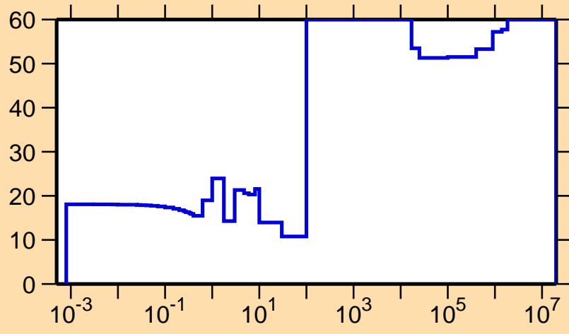
\Delta\sigma/\sigma vs. E for ^{162}\text{Yb}(n,\gamma)
