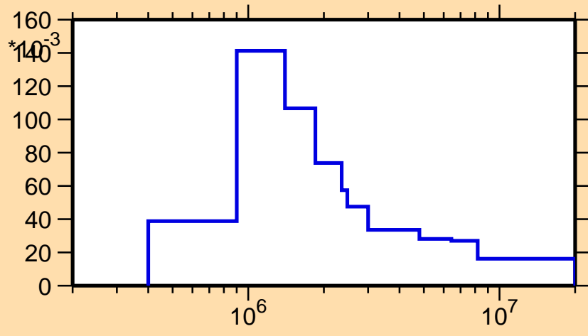
\sigma vs. E for ^{162}\text{Yb}(n,n_2)
