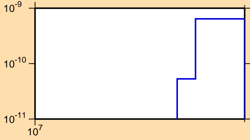
\sigma vs. E for ^{163}\text{Yb} (mt 45)
