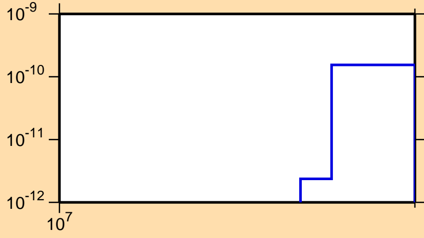
\sigma vs. E for ^{163}\text{Yb} (mt 34)
