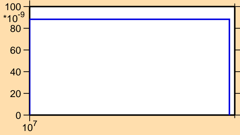
\sigma vs. E for ^{163}\text{Yb}(n,\text{nd})
