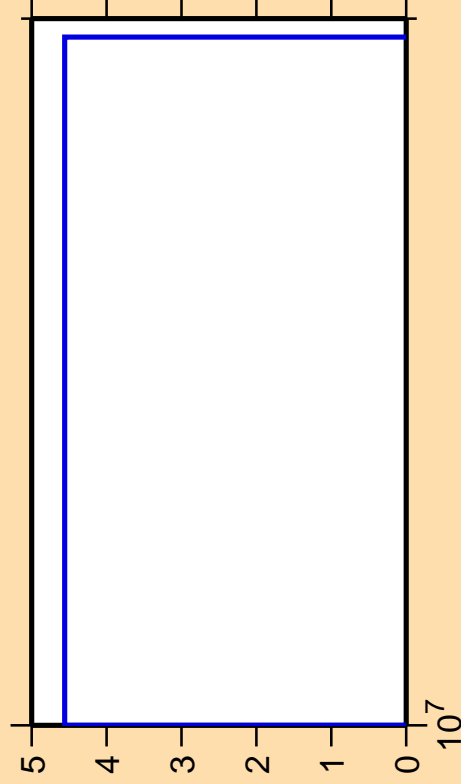
\Delta\sigma/\sigma vs. E for ^{163}\text{Yb} (mt 34)
