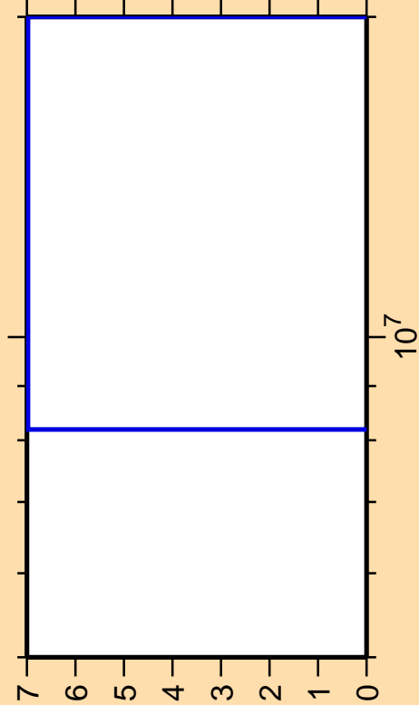
\Delta\sigma/\sigma vs. E for ^{163}\text{Yb} (mt 45)
