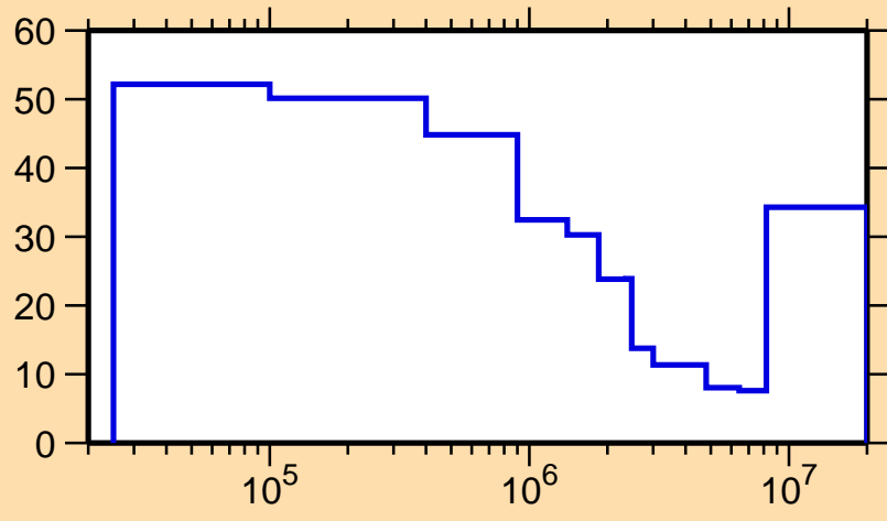
\Delta\sigma/\sigma vs. E for ^{163}\text{Yb}(n,\text{inel.})
