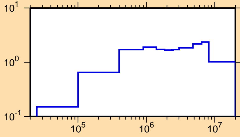
\sigma vs. E for ^{163}\text{Yb}(n,\text{inel.})
