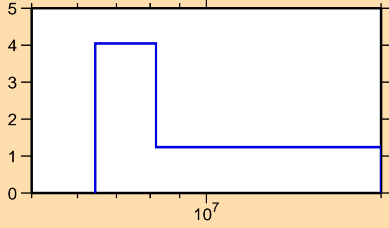
\Delta\sigma/\sigma vs. E for ^{163}\text{Yb}(n,\text{tot.})
