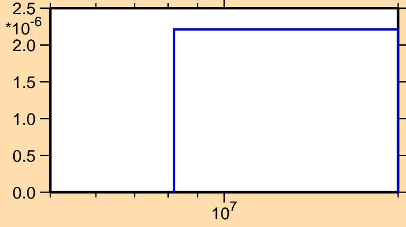
\sigma vs. E for ^{163}\text{Yb}(n,2n\alpha)
