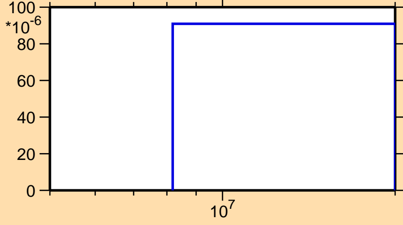
\sigma vs. E for ^{163}\text{Yb}(n,t)
