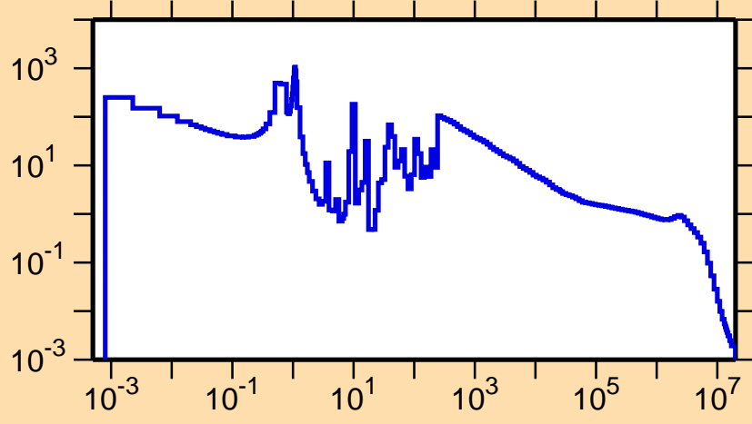
\sigma vs. E for ^{164}\text{Yb}(n,\gamma)
