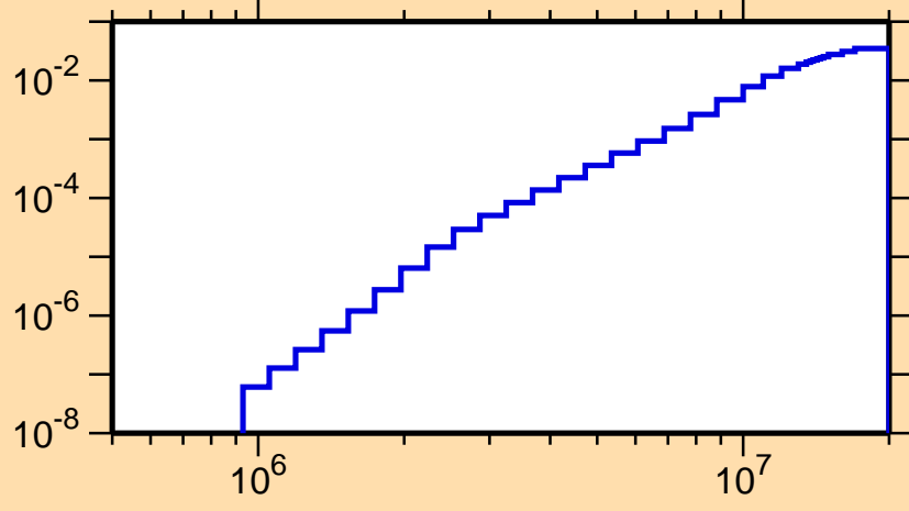
\sigma vs. E for ^{164}\text{Yb}(n,p)
