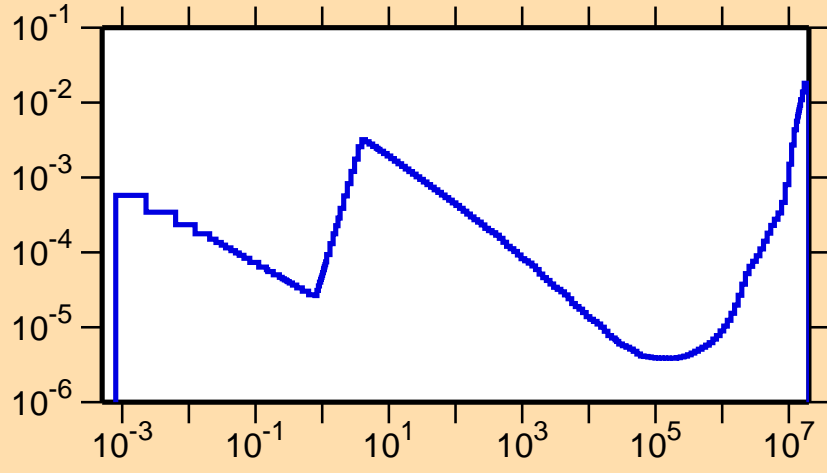
\sigma vs. E for ^{164}\text{Yb}(n,\alpha)
