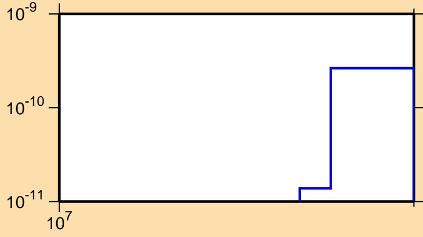
\sigma vs. E for ^{164}\text{Yb} (mt 45)
