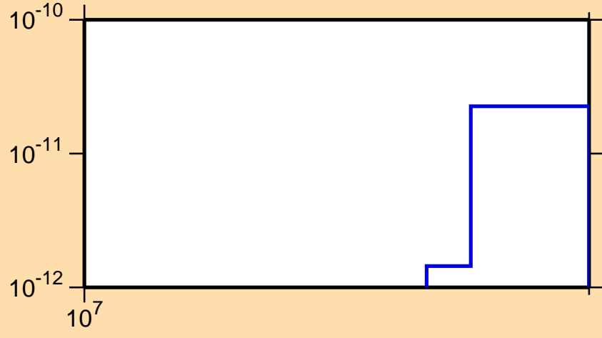
\sigma vs. E for ^{164}\text{Yb}(\text{mt117})
