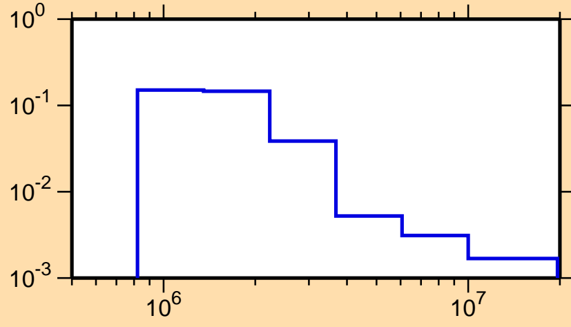
\sigma vs. E for ^{164}\text{Yb}(n,n_4)
