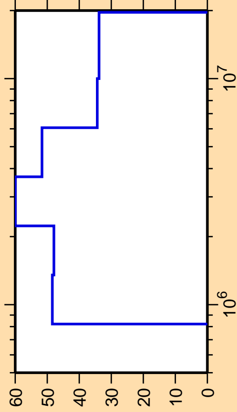
\Delta\sigma/\sigma vs. E for ^{164}\text{Yb}(n,n_4)
