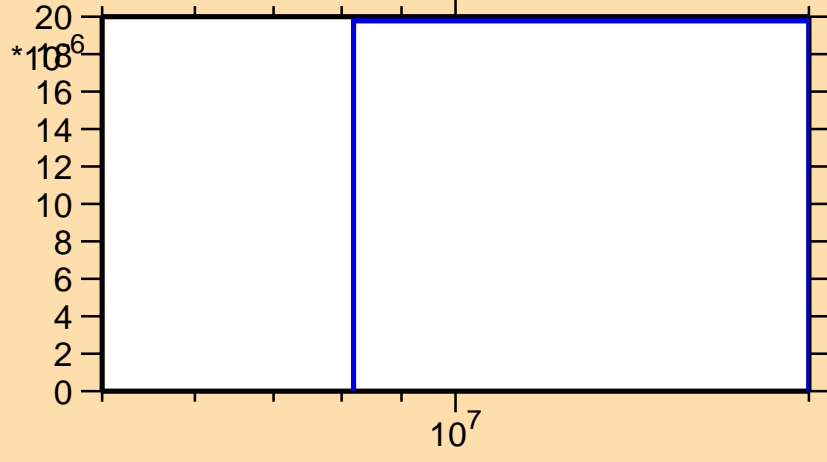
\sigma vs. E for ^{164}\text{Yb}(n,t)
