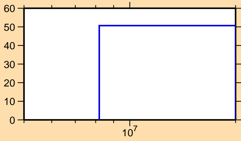
\Delta\sigma/\sigma vs. E for ^{164}\text{Yb}(n,2n)
