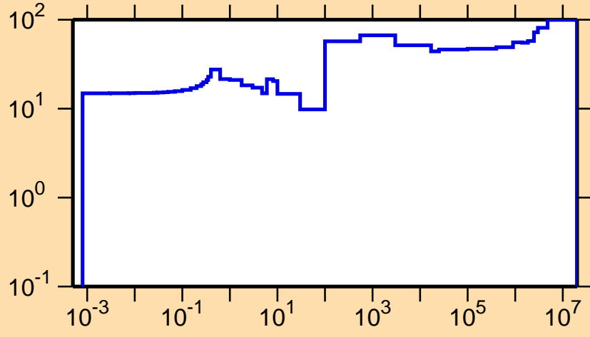
\Delta\sigma/\sigma vs. E for ^{164}\text{Yb}(n,\gamma)
