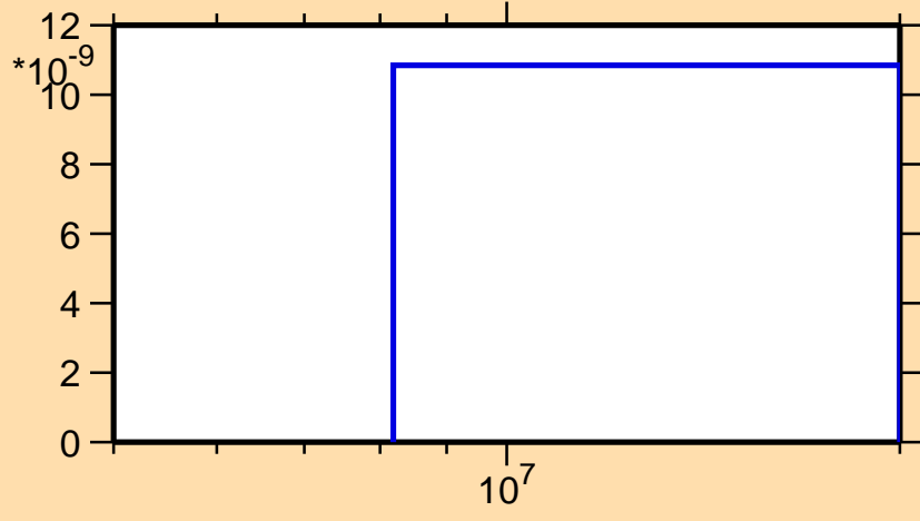
\sigma vs. E for ^{164}\text{Yb}(n,p\alpha)
