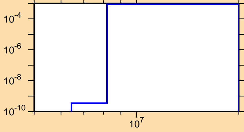
\sigma vs. E for ^{164}\text{Yb}(n,d)
