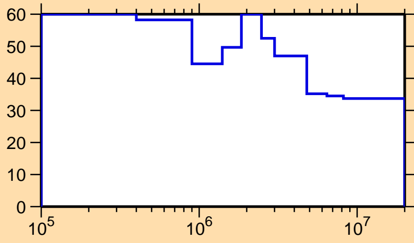
\Delta\sigma/\sigma vs. E for ^{164}\text{Yb}(n,n_1)
