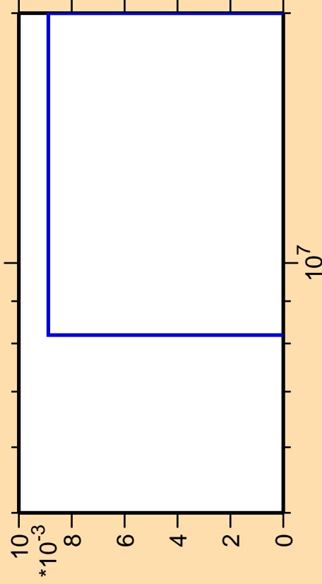
\Delta\sigma/\sigma vs. E for ^{164}\text{Yb} (mt 34)
