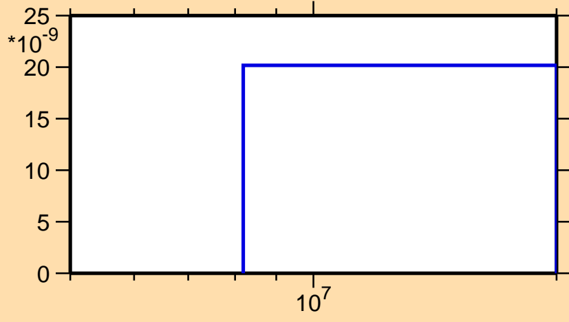
\sigma vs. E for ^{164}\text{Yb}(n,2n\alpha)
