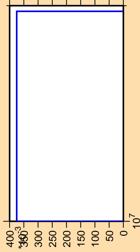
\Delta\sigma/\sigma vs. E for ^{165}\text{Yb} (mt 45)
