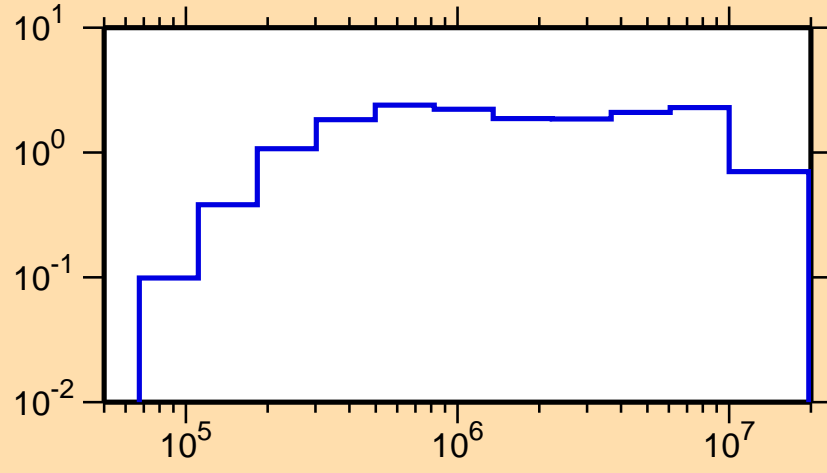
\sigma vs. E for ^{165}\text{Yb}(n,\text{inel.})
