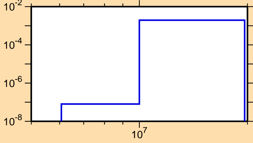
\sigma vs. E for ^{165}\text{Yb}(n,d)
