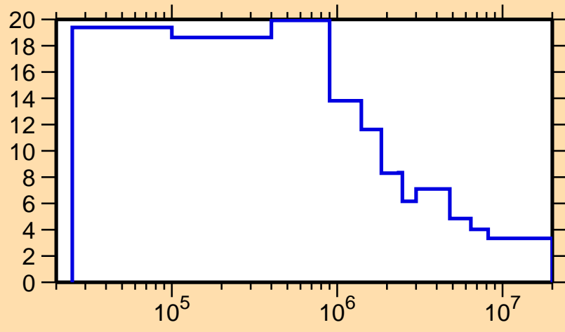
\Delta\sigma/\sigma vs. E for ^{165}\text{Yb}(n,\text{nonel.})
