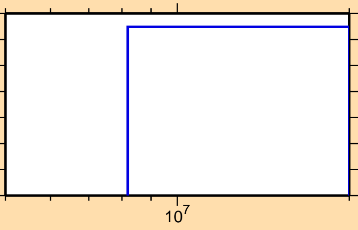
\sigma vs. E for ^{165}\text{Yb}(n,\text{nd})
