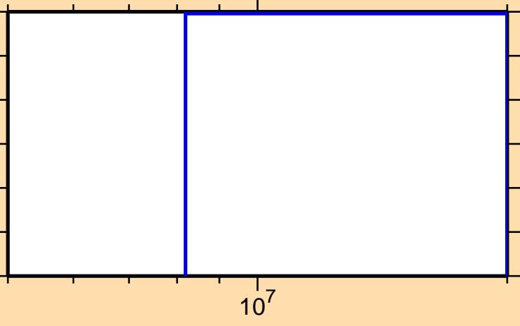
\sigma vs. E for ^{165}\text{Yb}(n,3n)
