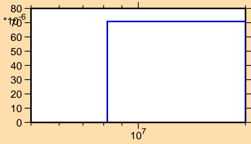
\sigma vs. E for ^{165}\text{Yb}(n,t)
