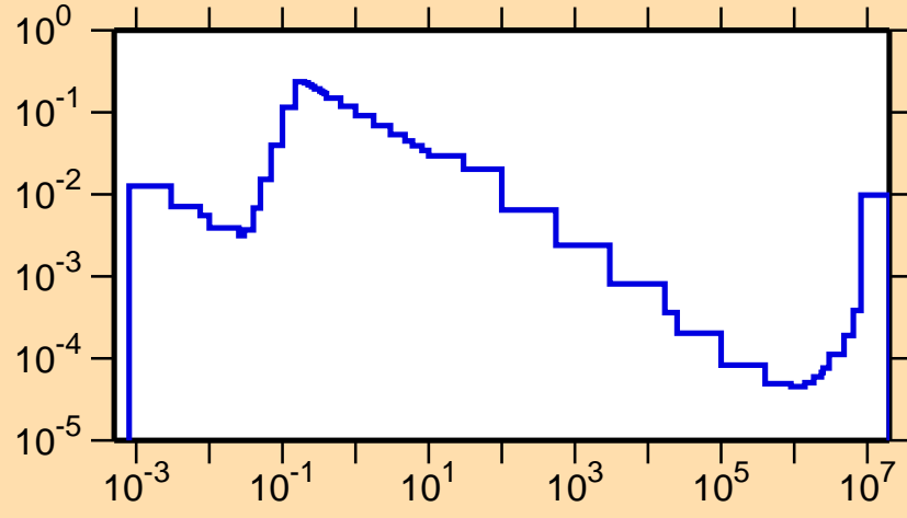
\sigma vs. E for ^{165}\text{Yb}(n,\alpha)
