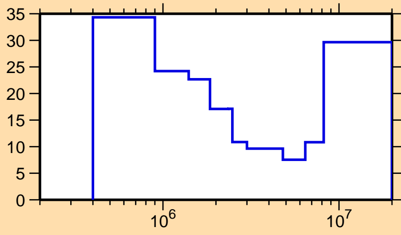
\Delta\sigma/\sigma vs. E for ^{165}\text{Yb}(n,n\text{cont.})
