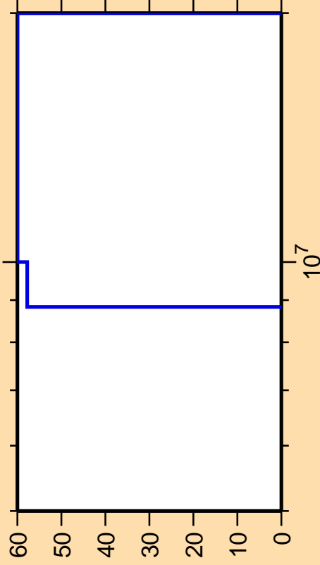
\Delta\sigma/\sigma vs. E for ^{166}\text{Yb}(n,n\text{cont.})
