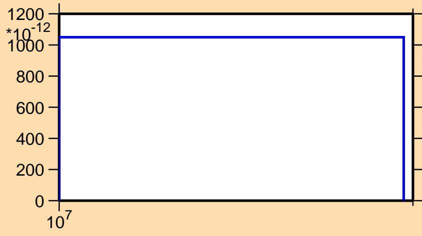
\sigma vs. E for ^{166}\text{Yb}(n,\text{He}3)
