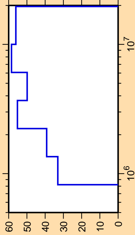
\Delta\sigma/\sigma vs. E for ^{166}\text{Yb}(n,n_4)
